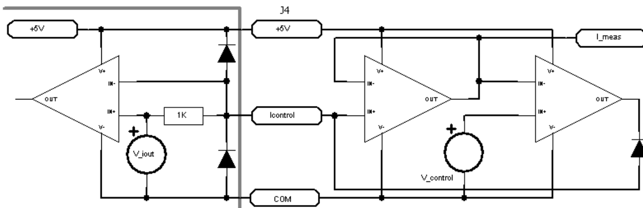
Measuring & controlling output current
