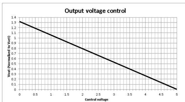
Control function
