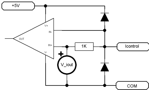
Equivalent internal circuit
