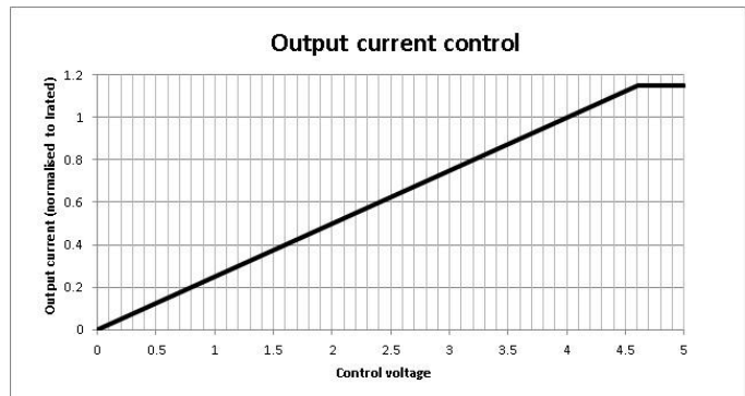
Control function
