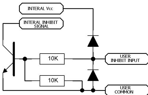
Internal circuit
