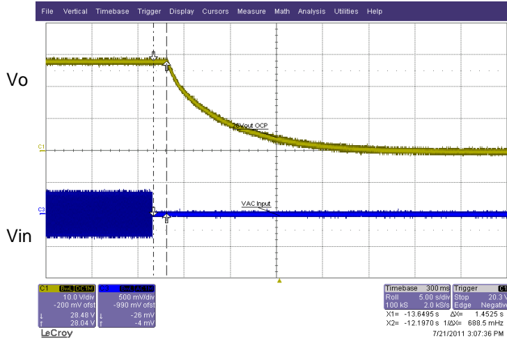
Output fall (0% load, 115Vac input)
