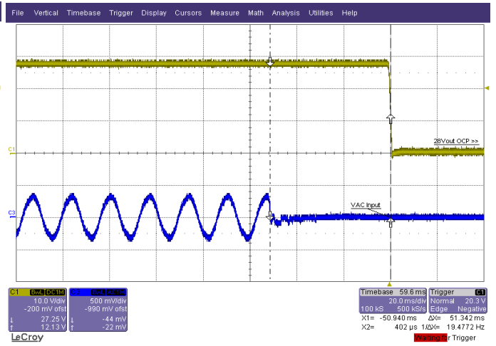
Output fall (100% load, 115Vac input)
