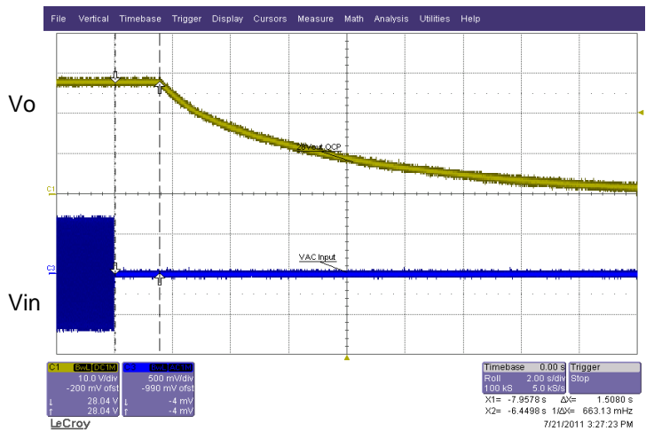
Output fall (0% load, 230Vac input)
