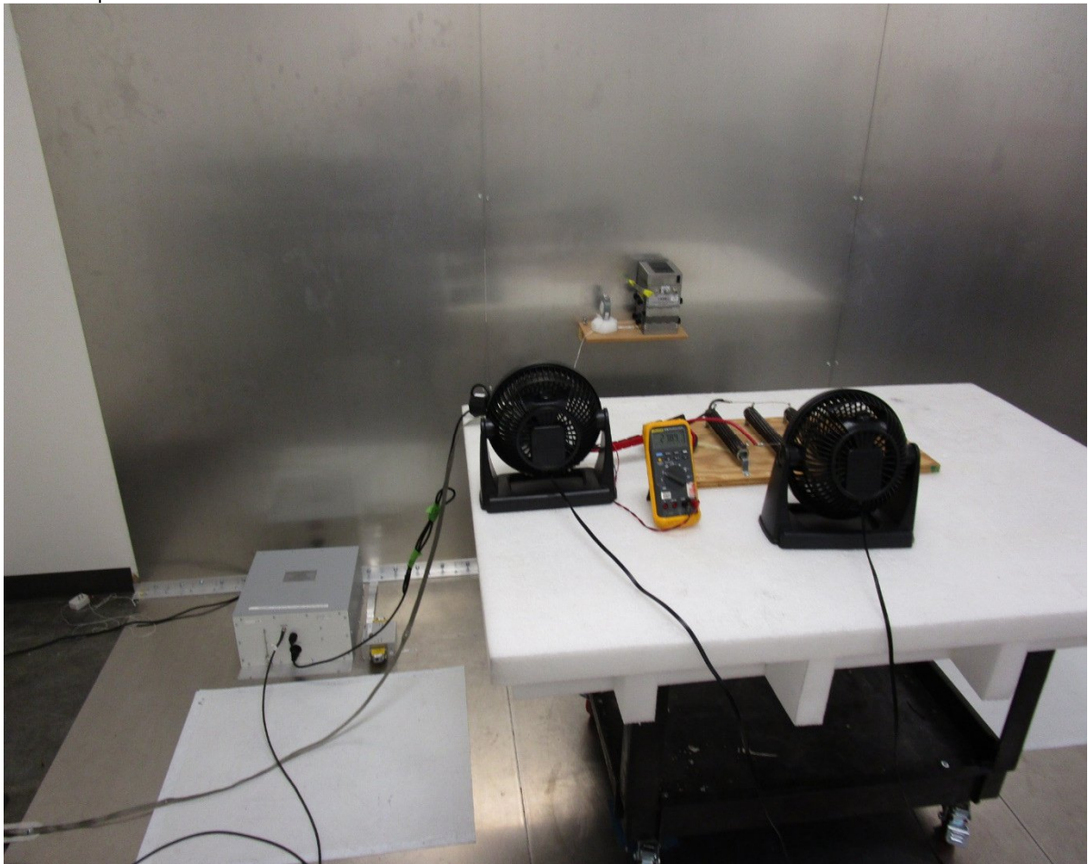
Test Setup
