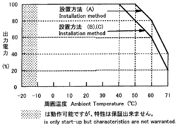
Fig.2 Output power vs. Ambient temperature
