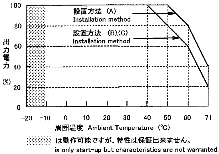
Fig.2 Output power vs. Ambient temperature
