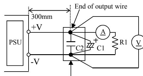
Figure A measurement setup
