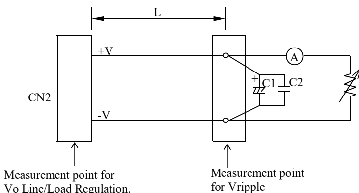
Fig A L: 150mm AWG#22 C1: Elec. Cap 100μF C2: Film Cap 0.1μF Bandwidth of scope: 100MHz
