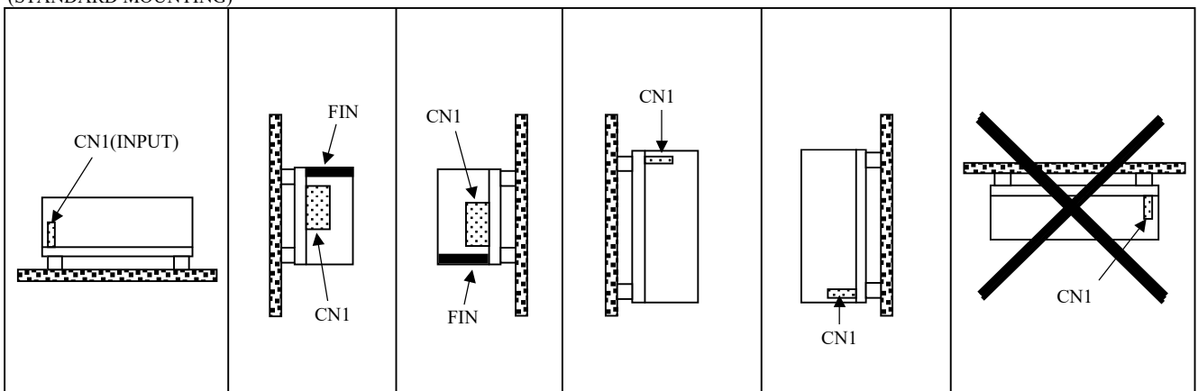
MOUNTING A
