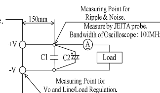
Fig. A C1 : Film Cap. 0.1 μF C2 : Elect. Cap. 100 μF
