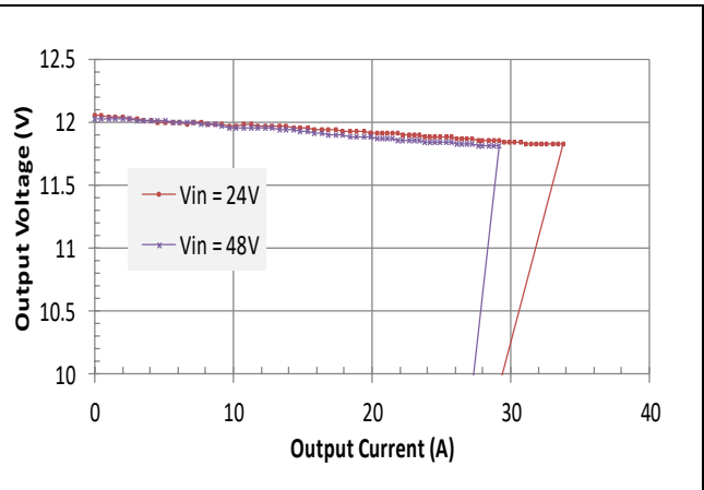
Vo = 12V Typical Current Limit Characteristics.
