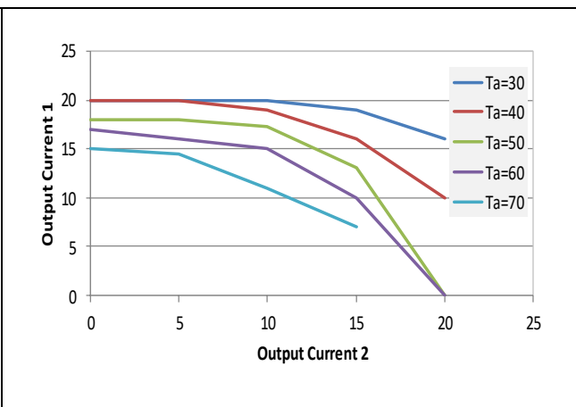
Vo1 = 12V Vo2 = 5V, Vin = 24V Output Current1 vs. Output Current2 at various ambient temperatures with NC (60lfm) airflow.
