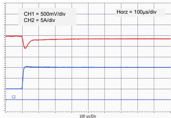
Vo = 12V Typical output voltage transient response to load step from 25% to 75% of full load with output current slew rate of 1A/µs.
