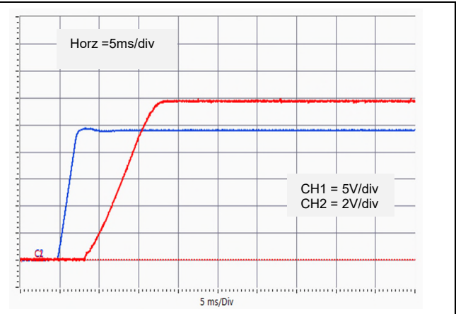
Vo = 12V Typical startup characteristic from input voltage at full load. Ch1 - input voltage, Ch2 – output voltage.
