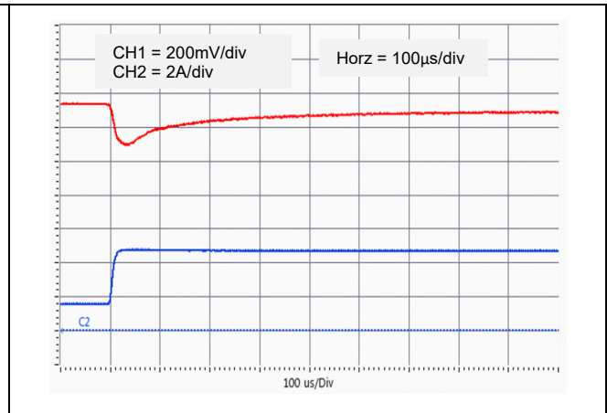
Vo2 = -12V Typical output voltage transient response to load step from 25% to 75% of full load with output current slew rate of 1A/μs.
