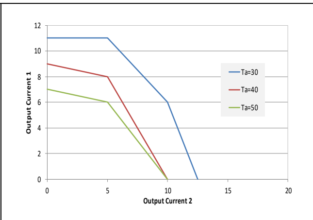
Vo1 = Vo2 = 12V, Vin = 53V output current1 vs. output current 2 at various ambient temperatures with NC (60lfm) airflow.
