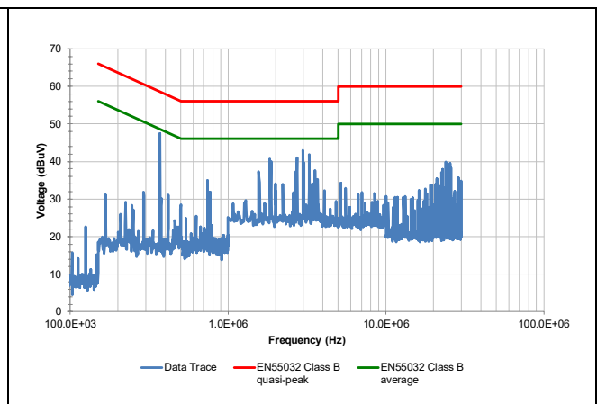
Typical Conducted Emissions V_{in} = 53V , V_o = 12V , full load.
