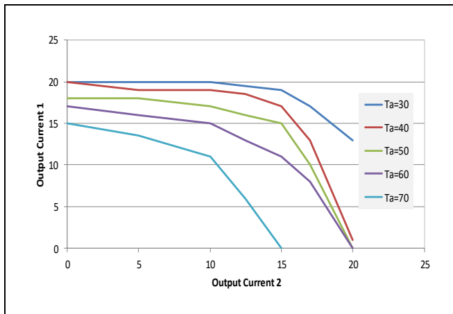
Vo1 = Vo2 = 12V, Vin = 24V Output Current1 vs. Output Current2 at various ambient temperatures with NC (60lfm) airflow.
