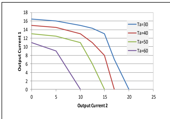
Vo1 = Vo2 = 12V, Vin = 36V Output Current1 vs. Output Current2 at various ambient temperatures with NC (60lfm) airflow.
