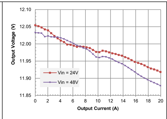
Vo = 12V Typical load regulation.
