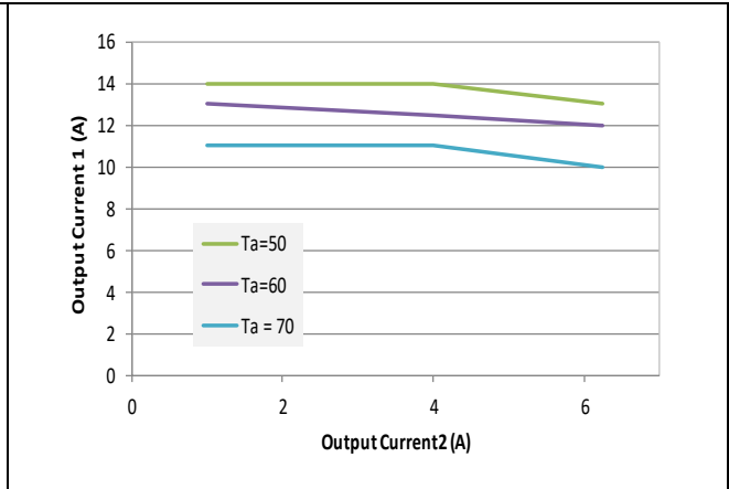
Vo1 = 12,Vo2 = -12V, Vin = 36V Output Current1 vs. Output Current2 at various ambient temperatures with NC (60lfm) airflow.
