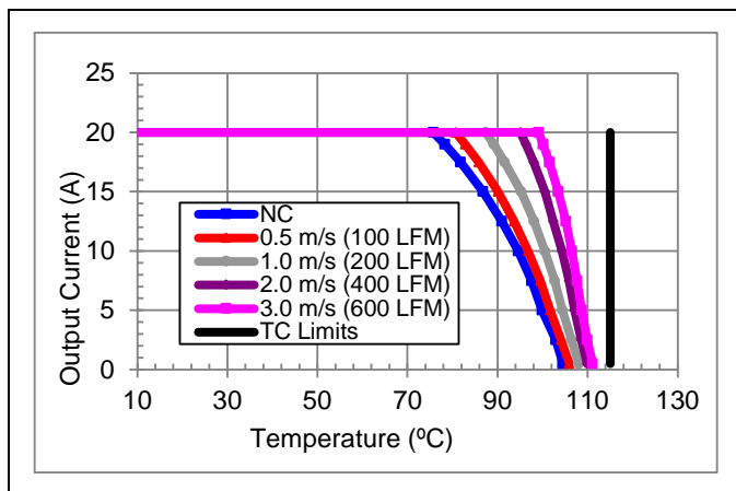
Vin = 48V, Vo = 5V preliminary maximum output current vs. ambient temperature for natural convection NC (60lfm) to 3m/s (600 lfm) with airflow from pin 3 to pin 4.
