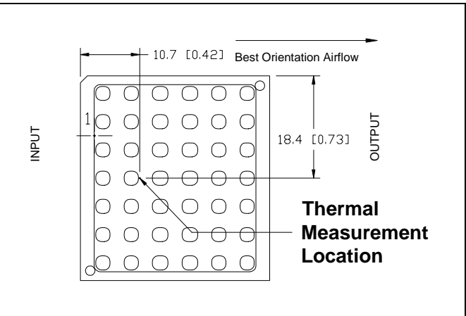
i7A12060A008V-xFx-R thermal measurement location – top view.
