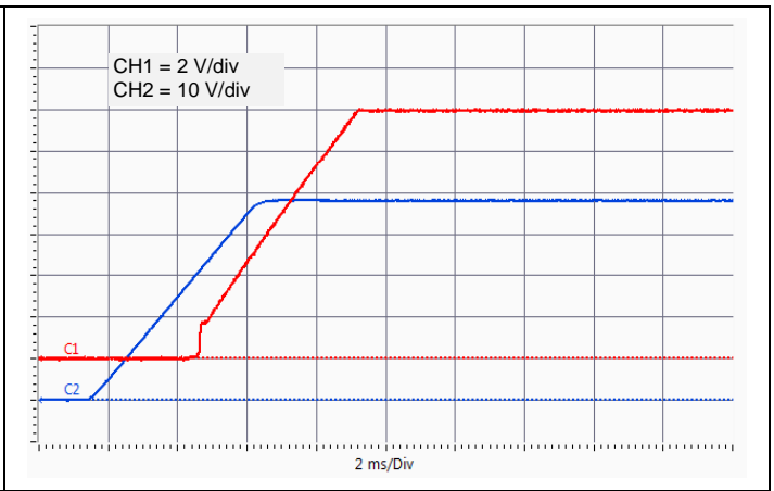
Vo = 12V Typical startup characteristic from input voltage at full load. CH1: Output Voltage, CH2: Input Voltage.
