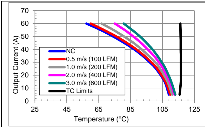
V_{in} = 12V , V_o = 1.8V preliminary maximum output current vs. ambient temperature for natural convection NC (60lfm) to 3m/s (600 lfm) with airflow from pin 3 to pin 4.
