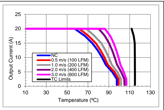
Vin = 48V, Vo = 24V preliminary maximum output current vs. ambient temperature for natural convection NC (60lfm) to 3m/s (600 lfm) with airflow from pin 3 to pin 4.
