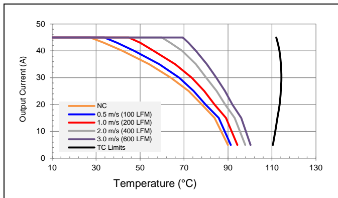
Vin = 24V, Vo = 12V preliminary maximum output current vs. ambient temperature for natural convection NC (60lfm) to 3m/s (600 lfm) with airflow from pin 3 to pin 4.
