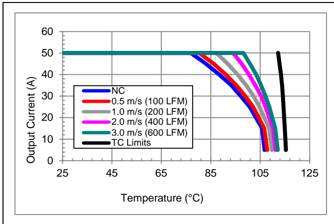
Vin = 12V, Vo = 8V preliminary maximum output current vs. ambient temperature for natural convection NC (60lfm) to 3m/s (600 lfm) with airflow from pin 3 to pin 4.
