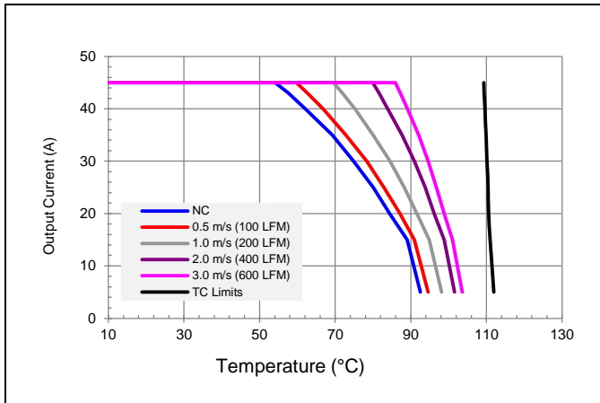
V_{in} = 24V , V_o = 15V preliminary maximum output current vs. ambient temperature for natural convection NC (60lfm) to 3m/s (600 lfm) with airflow from pin 3 to pin 4.
