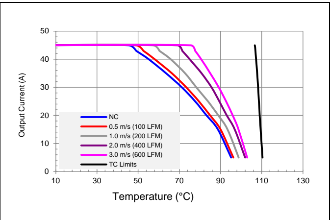
V_{in} = 24V , V_o = 5V preliminary maximum output current vs. ambient temperature for natural convection NC (60lfm) to 3m/s (600 lfm) with airflow from pin 3 to pin 4.
