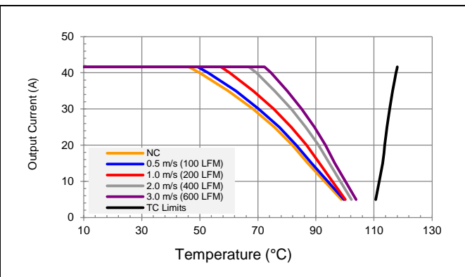
Vin = 24V, Vo = 18V preliminary maximum output current vs. ambient temperature for natural convection NC (60lfm) to 3m/s (600 lfm) with airflow from pin 3 to pin 4.
