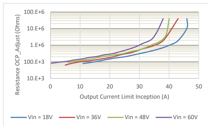
Typical OCP adjustment of i7A4W033A033V module with Vout = 15V
