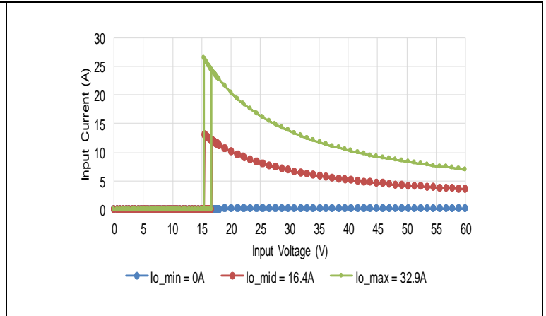
V_o = 12V Typical Input Current vs. Input Voltage Characteristics.
