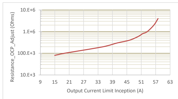
Typical i7A12060A008V OCP adjustment with Vin = 12V, Vout = 8V
