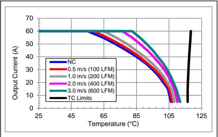
Vin = 12V, Vo = 3.3V preliminary maximum output current vs. ambient temperature for natural convection NC (60lfm) to 3m/s (600 lfm) with airflow from pin 3 to pin 4.
