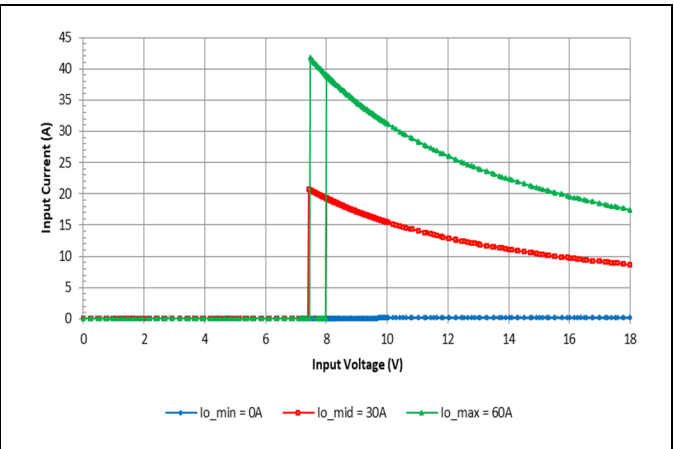
Vo = 5V Typical Input Current vs. Input Voltage Characteristics.
