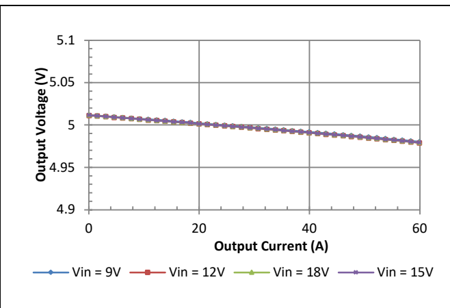
Vo = 5V Typical Load regulation.
