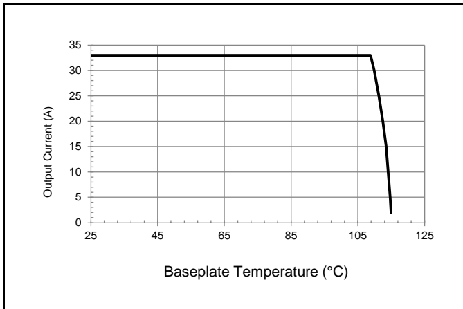
Typical baseplate temperature versus output current derating curve for conduction cooling application with Vo = 12V
