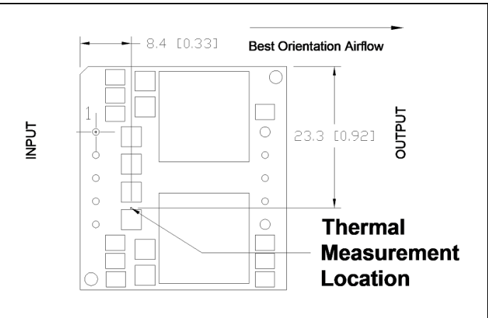
i7A48020A033V thermal measurement location – top view.
