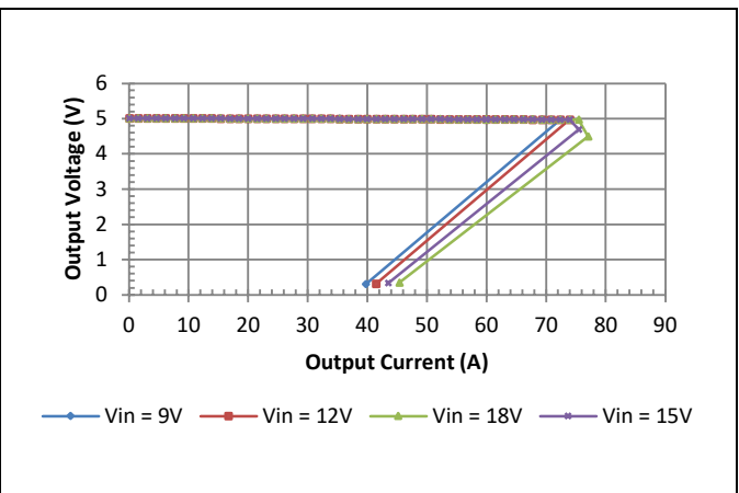
Vo = 5V Typical Current Limit Characteristics.
