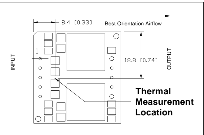
i7A4W033A033V thermal measurement location – top view.
