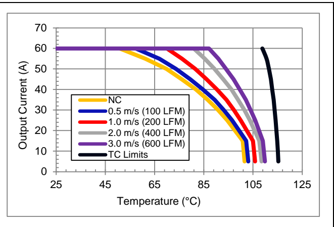
Vin = 18V, Vo = 5V preliminary maximum output current vs. ambient temperature for natural convection NC (60lfm) to 3m/s (600 lfm) with airflow from pin 3 to pin 4.
