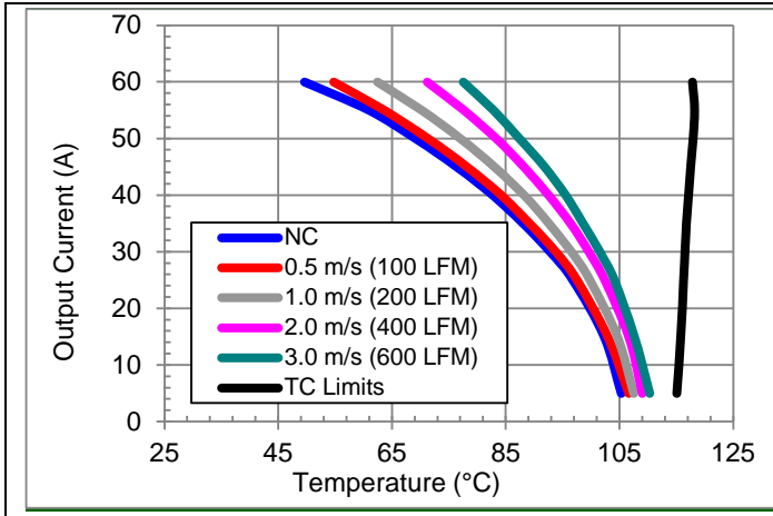
V_{in} = 12V , V_o = 5V preliminary maximum output current vs. ambient temperature for natural convection NC (60lfm) to 3m/s (600 lfm) with airflow from pin 3 to pin 4.
