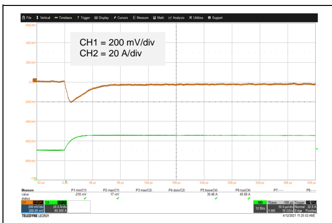
Vo = 3.3V Typical output voltage transient response to load step from 50% to 75% of full load with output current slew rate of 1A/ \mu s, Cext = 330 \mu F.
