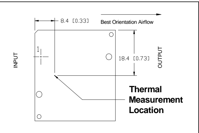
i7A48020A033V-xCx-R thermal measurement location – top view.
