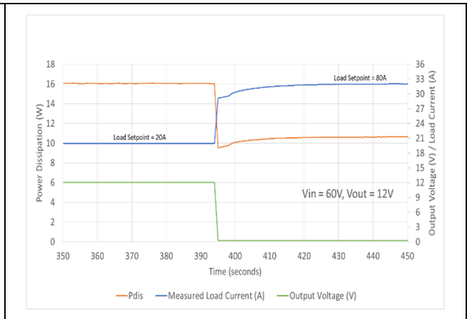
V_{in} = 60V Typical overload characteristics.
