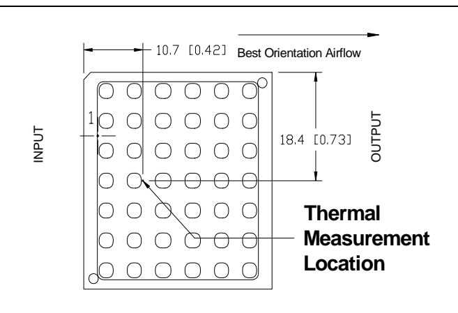
i7A4W020A033V-xFx-R thermal measurement location – top view.
