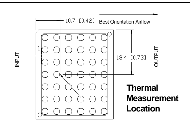
i7A4W033A033V-xFx-R thermal measurement location – top view.
