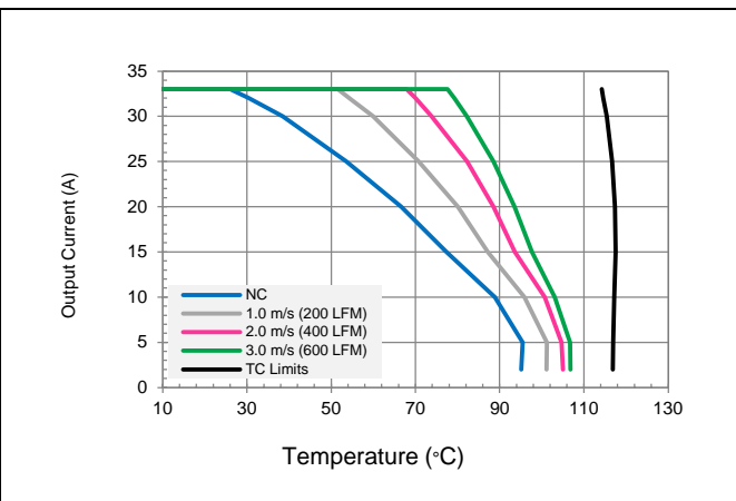
V_{in} = 48V , V_o = 12V preliminary maximum output current vs. ambient temperature for natural convection NC (60lfm) to 3m/s (600 lfm) with airflow from pin 3 to pin 4.
