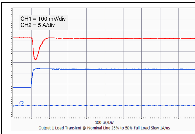
V_o = 12V Typical output voltage transient response to load step from 25% to 50% of full load with output current slew rate of 1A/\mu s , C_{ext} = 240 \mu F .
