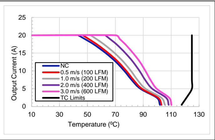
V_{in} = 60V , V_o = 12V preliminary maximum output current vs. ambient temperature for natural convection NC (60lfm) to 3m/s (600 lfm) with airflow from pin 3 to pin 4.
