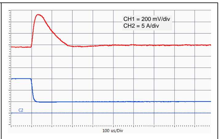
Vo = 12V Typical output voltage transient response to load step from 75% to 25% of full load with output current slew rate of 1A/ \mu s, Cext = 330 \mu F capacitor.
