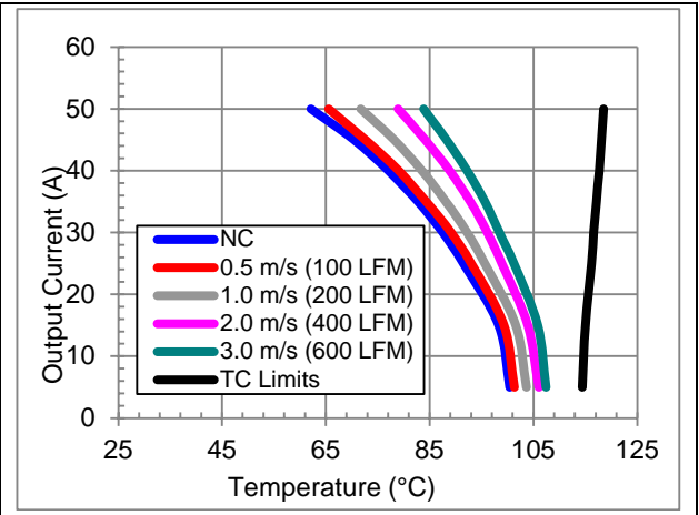
V_{in} = 15V , V_o = 8V preliminary maximum output current vs. ambient temperature for natural convection NC (60lfm) to 3m/s (600 lfm) with airflow from pin 3 to pin 4.
