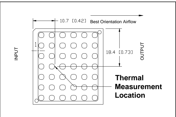
i7A24045A033V-xFx-R thermal measurement location – top view.
