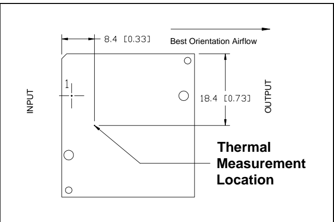
i7A24045A033V-xCx-R thermal measurement location – top view.
