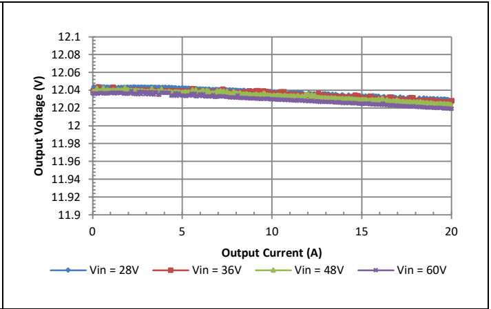
Vo = 12V typical load regulation
