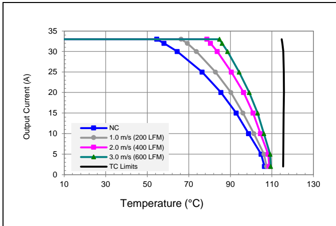
Vin = 24V, Vo = 12V preliminary maximum output current vs. ambient temperature for natural convection NC (60lfm) to 3m/s (600 lfm) with airflow from pin 3 to pin 4.
