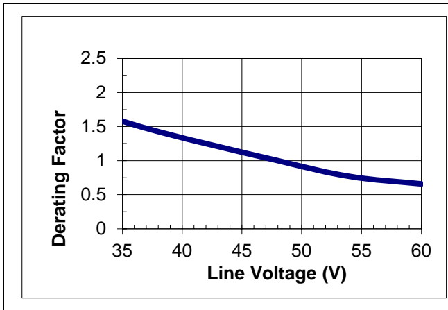
Typical output current derating versus line voltage with airflow 1m/s (200 lfm) and T_a = 65^\circ C .
