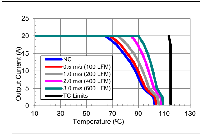
Vin = 48V, Vo = 12V preliminary maximum output current vs. ambient temperature for natural convection NC (60lfm) to 3m/s (600 lfm) with airflow from pin 3 to pin 4.
