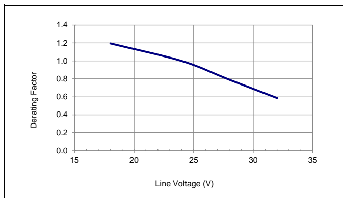
Typical output current derating versus line voltage with airflow 1m/s (200 lfm) and Ta = 65 °C.
