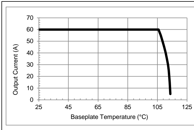
Typical Baseplate temperature versus output current derating curve for conduction cooling application with Vo = 5V.
