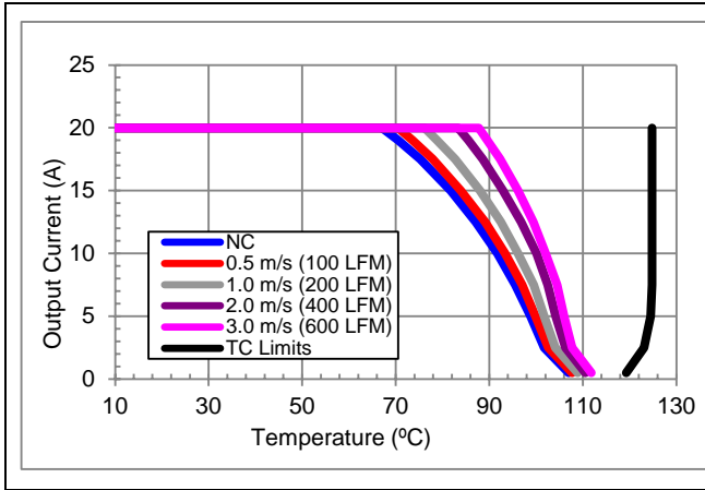
V_{in} = 48V , V_o = 5V preliminary maximum output current vs. ambient temperature for natural convection NC (60lfm) to 3m/s (600 lfm) with airflow from pin 3 to pin 4.
