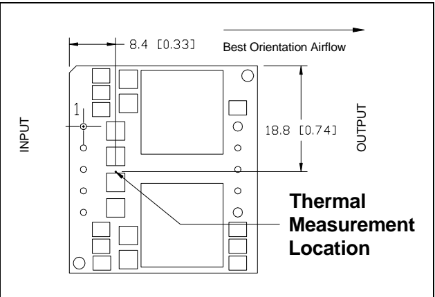
i7A12060A008V thermal measurement location – top view.
