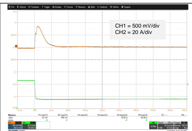
Vo = 3.3V Typical output voltage transient response to load step from 75% to 25% of full load with output current slew rate of 1A/ \mu s, Cext = 330 \mu F capacitor.
