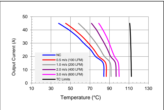
V_{in} = 32V , V_o = 15V preliminary maximum output current vs. ambient temperature for natural convection NC (60lfm) to 3m/s (600 lfm) with airflow from pin 3 to pin 4.
