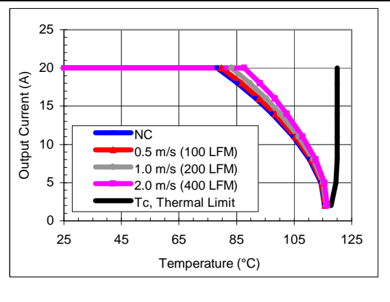
V_o=1.8V , V_{in}=3.3V maximum output current vs. ambient temperature at nominal input voltage for natural convection (60lfm) to 400lfm with airflow from pin 3 to pin 7.
