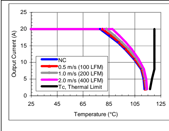
V_o=3.3V , V_{in}=5V maximum output current vs. ambient temperature at nominal input voltage for natural convection (60lfm) to 400lfm with airflow from pin 3 to pin 7.
