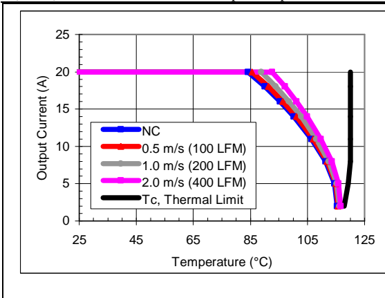
V_o=0.6V , V_{in}=3.3V maximum output current vs. ambient temperature at nominal input voltage for natural convection (60lfm) to 400lfm with airflow from pin 3 to pin 7.
