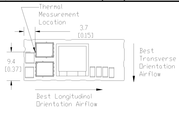
iAF05020A006V thermal measurement location – top view
