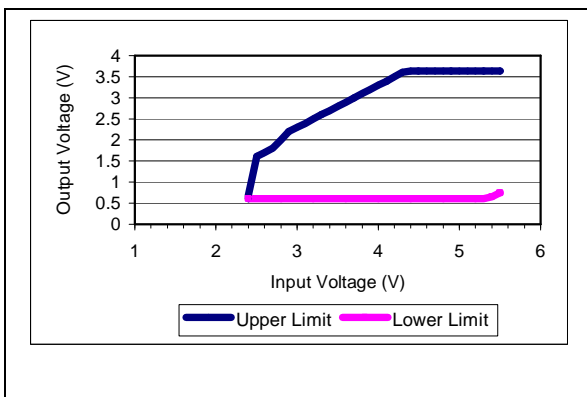
B Output Voltage versus Input Voltage Operating Range
