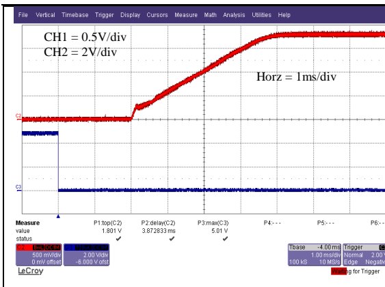
I_V=1.8V Typical startup characteristic from on/off at light load. Upper trace - output voltage, lower trace – on/off signal
