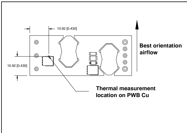
iEA48005A150V-000 thermal measurement location – top view
