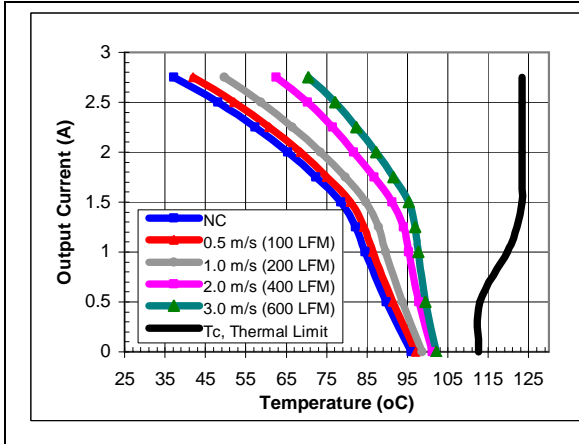
iEA48003A280V-000 maximum output current vs. ambient temperature at nominal input voltage for airflow rates natural convection (60lfm) to 600lfm with airflow from pin 3 to pin 1.
