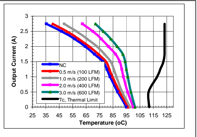
iEA48003A280V-000 maximum output current vs. ambient temperature at nominal input voltage for airflow rates natural convection (60lfm) to 600lfm with airflow from pin 1 to pin 3.
