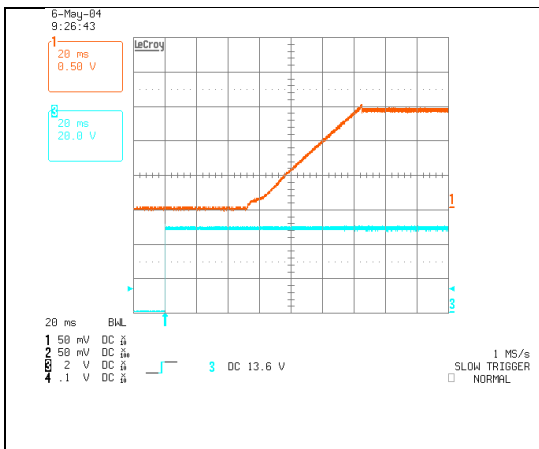
iEA48025A015V-000 Typical startup characteristic from input voltage application at full load. Ch3 - input voltage, Ch 1 – output voltage
