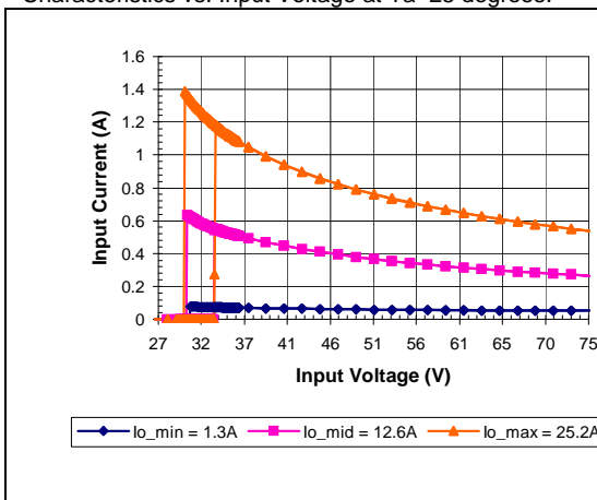
iEA48025A012V-000 Typical Input Current vs. Input Voltage Characteristics
