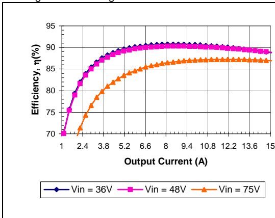
iEA48015A050V-000 Typical Efficiency vs. Input Voltage at Ta=85 degrees.
