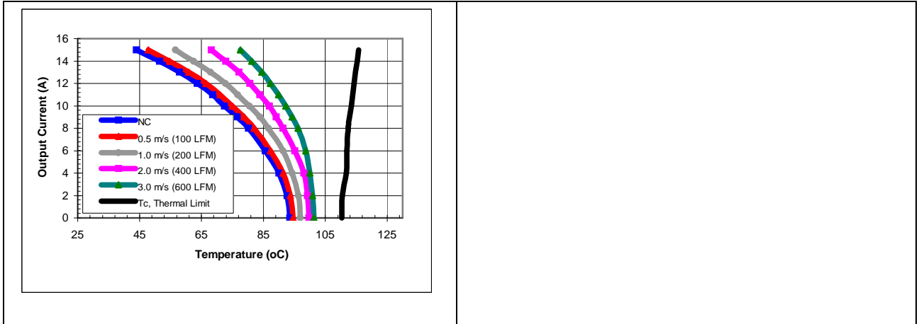
iEA48015A050V-000 maximum output current vs. ambient temperature at nominal input voltage for airflow rates natural convection (60lfm) to 600lfm with airflow from pin 3 to pin 1.
