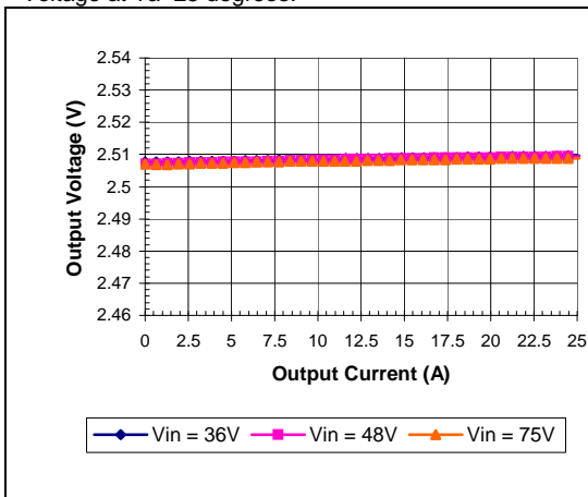
iEA48025A025V-000 Typical Output Voltage vs. Load Current at Ta = 25 degrees
