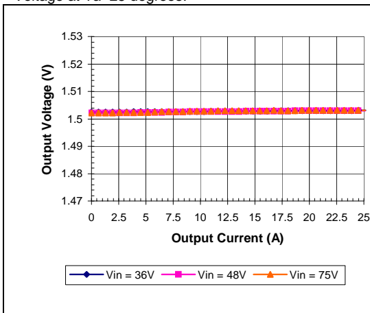
iEA48025A015V-000 Typical Output Voltage vs. Load Current at Ta = 25 degrees
