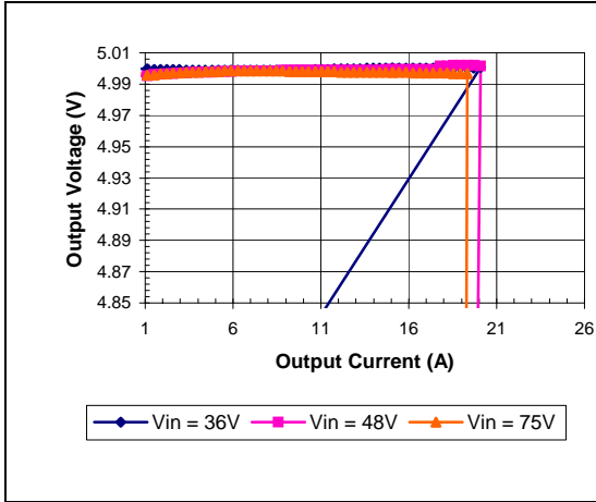
iEA48015A050V-000 Typical Output Current Limit Characteristics vs. Input Voltage at Ta=25 degrees.
