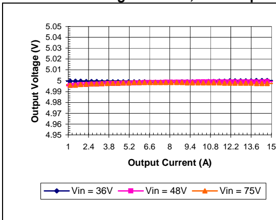
iEA48015A050V-000 Typical Output Voltage vs. Load Current at Ta = 25 degrees
