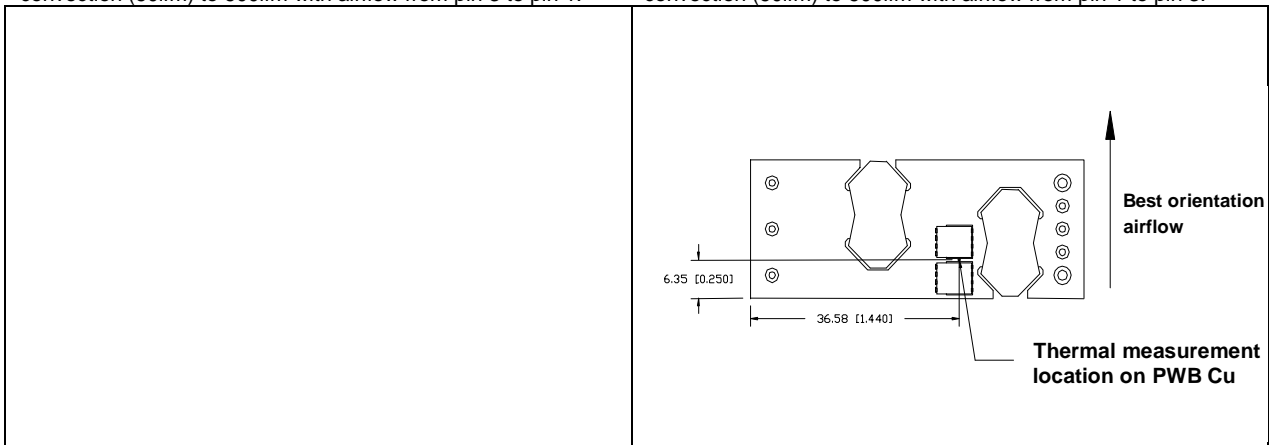
iEA48020A033V-000 thermal measurement location – top view
