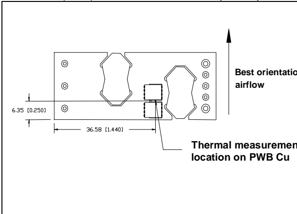
iEA48007A120V-000 thermal measurement location – top view
