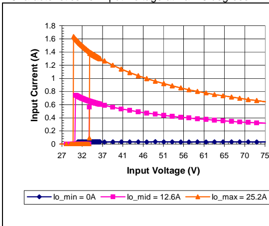
iEA48025A015V-000 Typical Input Current vs. Input Voltage Characteristics
