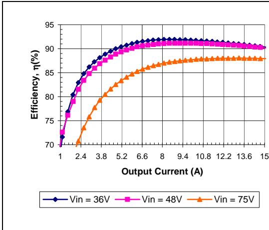
iEA48015A050V-000 Typical Efficiency vs. Input Voltage at Ta=25 degrees.
