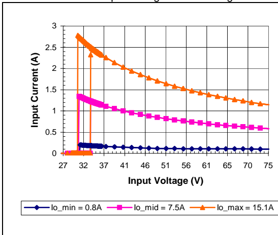
iEA48015A050V-000 Typical Input Current vs. Input Voltage Characteristics
