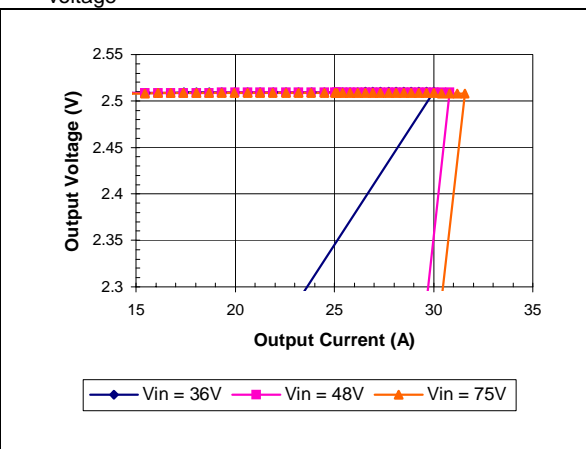
iEA48025A025V-000 Typical Output Current Limit Characteristics vs. Input Voltage at Ta=25 degrees.
