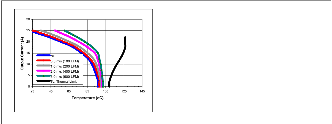
iEA48025A012V-000 maximum output current vs. ambient temperature at nominal input voltage for airflow rates natural convection (60lfm) to 600lfm with airflow from pin 3 to pin 1.
