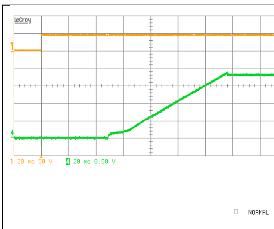
iEA48025A018V-000 Typical startup characteristic from input voltage application at full load. Ch1 - input voltage, Ch 4 – output voltage
