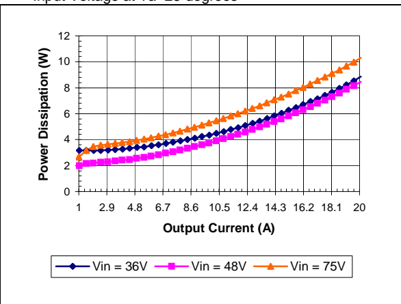
iEA48020A033V-000 Typical Power Dissipation vs. Input Voltage at Ta=85 degrees
