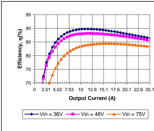
iEA48025A025V-000 Typical Efficiency vs. Input Voltage at Ta=25 degrees.
