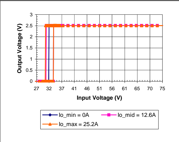
iEA48025A025V-000 Typical Output Voltage vs. Input Voltage Characteristics
