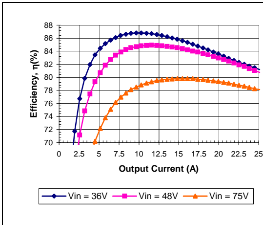
iEA48025A015V-000 Typical Efficiency vs. Input Voltage at Ta=25 degrees.
