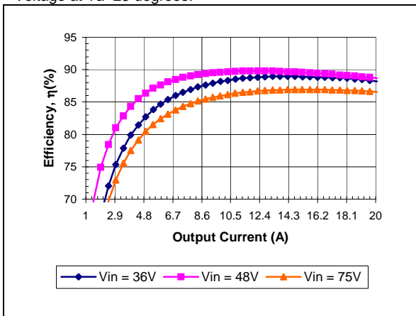
iEA48020A033V-000 Typical Efficiency vs. Input Voltage at Ta=85 degrees.
