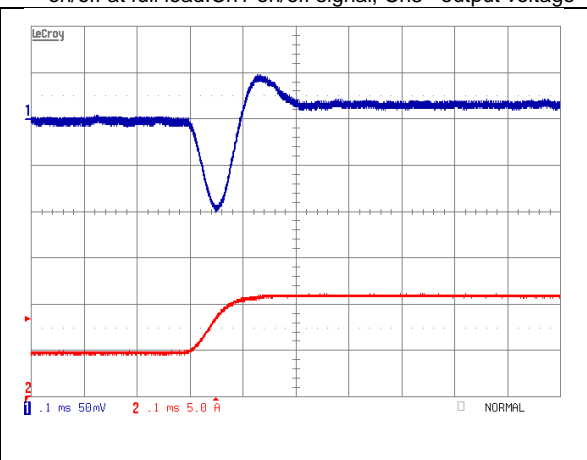
iEA48025A012V-000 Typical transient response. Output voltage response to load step from 50% to 75% of full load with output current slew rate of 0.1A/uS.
