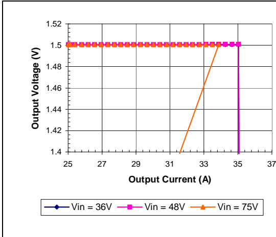
iEA48025A015V-000 Typical Output Current Limit Characteristics vs. Input Voltage at Ta=25 degrees.
