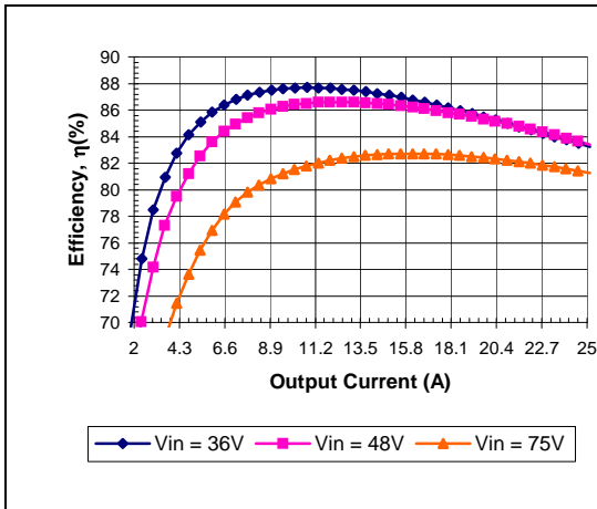
iEA48025A018V-000 Typical Efficiency vs. Input Voltage at Ta=25 degrees.
