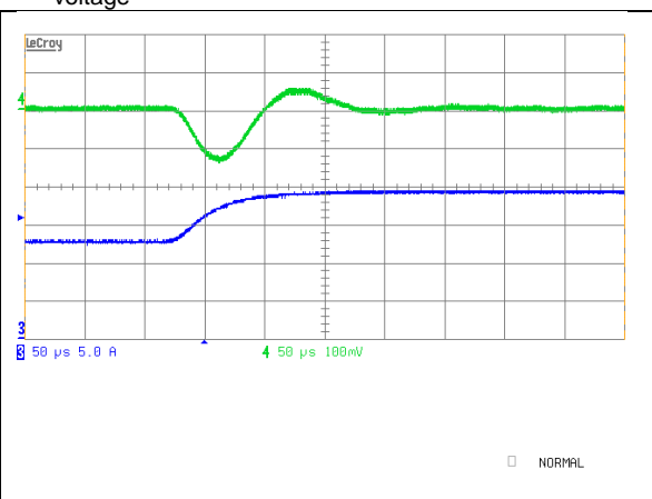
iEA48025A018V-000 Typical transient response. Output voltage response to load step from 50% to 75% of full load with output current slew rate of 0.1A/uS.
