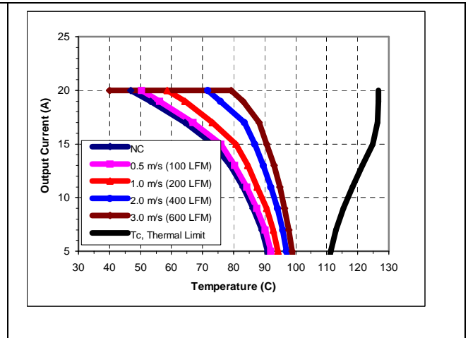
iEA48020A033V-000 maximum output current vs. ambient temperature at nominal input voltage for airflow rates natural convection (60lfm) to 600lfm with airflow from pin 1 to pin 3.
