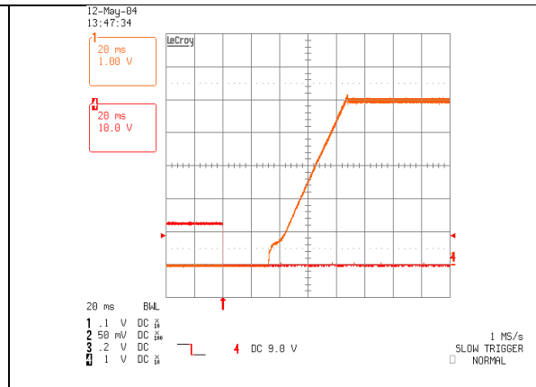
iEA48015A050V-001 Typical startup characteristic from on/off at full load. Ch4 - on/off signal, Ch 1 – output voltage
