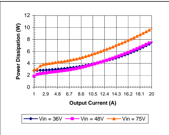
iEA48020A033V-000 Typical Power Dissipation vs. Input Voltage at Ta=25 degrees
