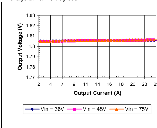
iEA48025A018V-000 Typical Output Voltage vs. Load Current at Ta = 25 degrees
