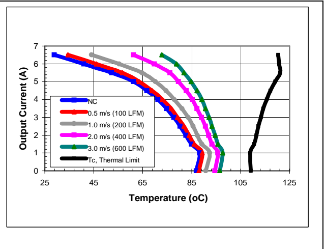
iEA48007A120V-000 maximum output current vs. ambient temperature at nominal input voltage for airflow rates natural convection (60lfm) to 600lfm with airflow from pin 1 to pin 3.
