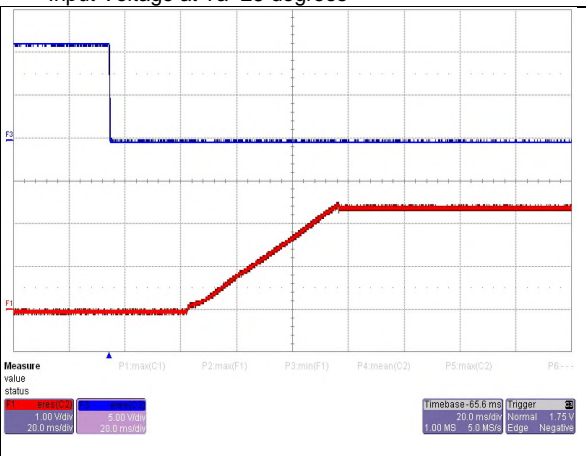
iEA48025A025V-001 Typical startup characteristic from on/off at full load. Ch3 - on/off signal, Ch 1 – output voltage
