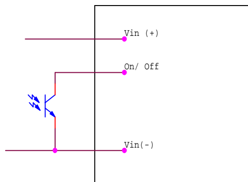
On/Off Circuit for positive or negative logic
