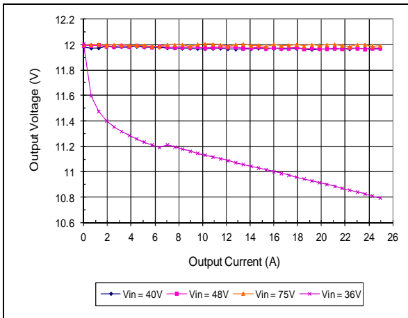
Typical Output Voltage vs. Load Current at Ta=25C (Droop Feature Disabled)
