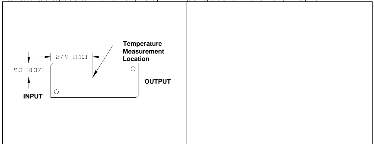
Thermal measurement location for base plate option – top view
