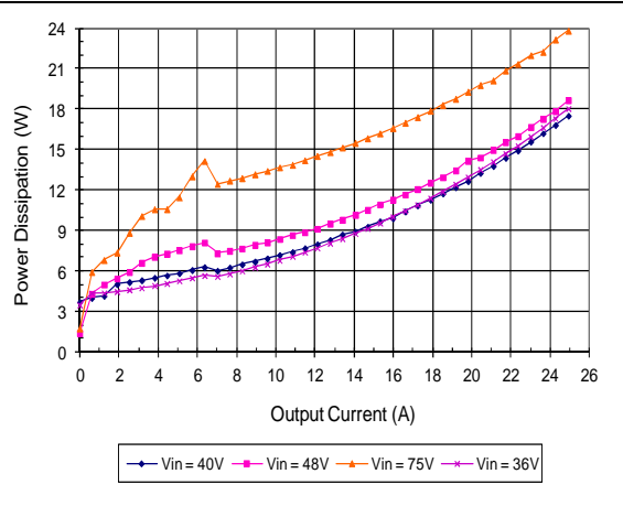
Power Dissipation at various lines and loads (test in socket, 25C)
