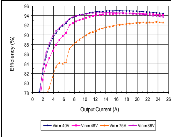
Efficiency at various lines and loads (test in socket, 25C)
