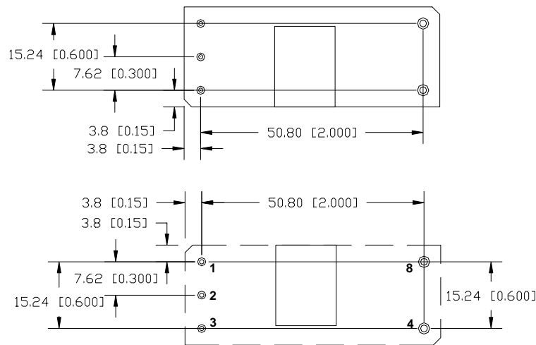
Recommended hole pattern (top view)
