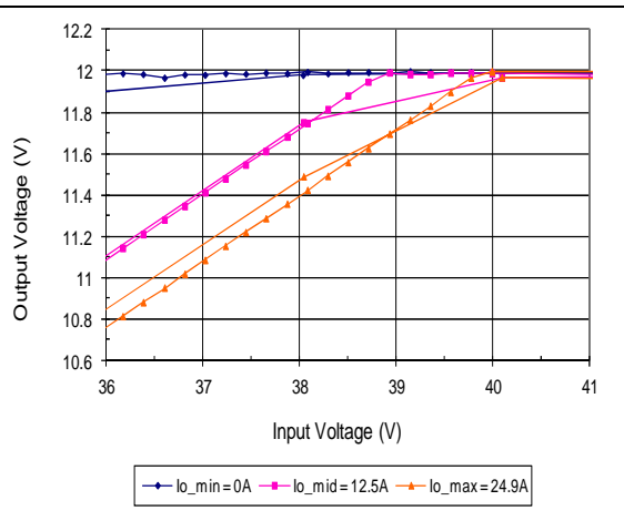
Output Voltage vs. Vin (between 36V and 41V)
