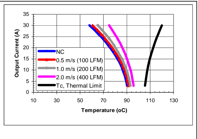
iQE24030A033V-000 maximum output current vs. ambient temperature at nominal input voltage for airflow rates natural convection (60lfm) to 400lfm with airflow from pin 1 to pin 3
