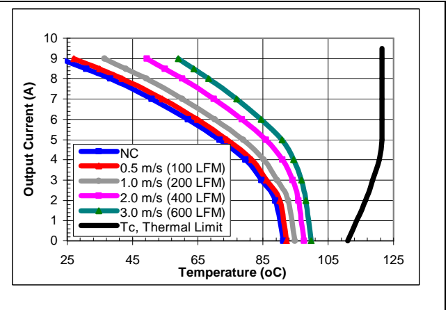
iQE24009A120V-000 maximum output current vs. ambient temperature at nominal input voltage for airflow rates natural convection (60lfm) to 600lfm with airflow from pin 1 to pin 3
