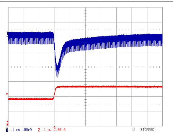
iQE24007A150V-000 Typical output voltage response to load step from 50% to 75% of full load with output current slew rate of 0.1A/uS. 100mV, 100uS per div.
