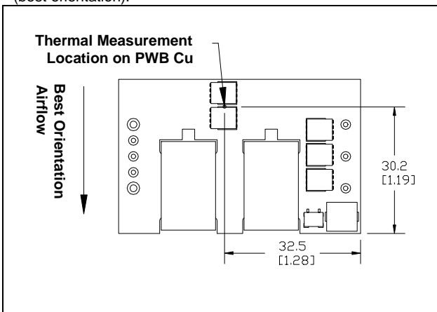
iQE24030A033V-000 thermal measurement location – top view
