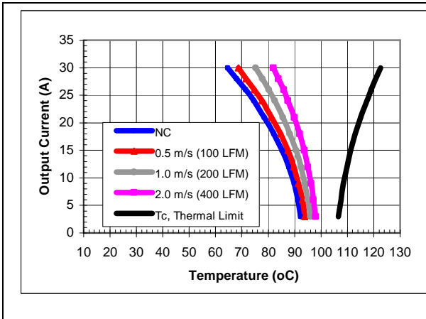
iQE24030A033V-000 maximum output current vs. ambient temperature at nominal input voltage for airflow rates natural convection (60lfm) to 400lfm with airflow from pin 3 to pin 1 (best orientation).
