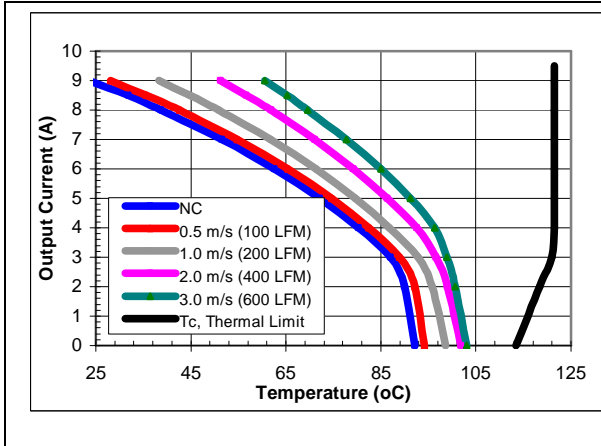
iQE24009A120V-000 maximum output current vs. ambient temperature at nominal input voltage for airflow rates natural convection (60lfm) to 600lfm with airflow from pin 3 to pin 1 (best orientation).
