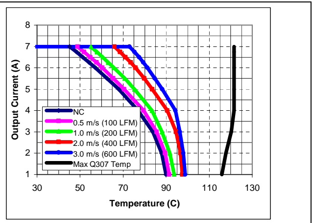
iQE24007A150V-000 maximum output current vs. ambient temperature at nominal input voltage for airflow rates natural convection (60lfm) to 600lfm with airflow from pin 1 to pin 3
