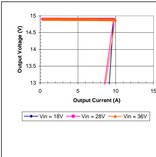
iQE24007A150V-000 Typical Output Current Limit Characteristics vs. Input Voltage at Ta=25 degrees.
