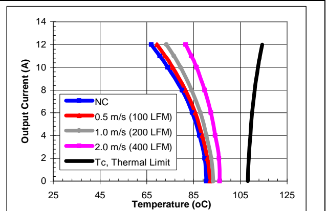
iQE24012A080V-000 maximum output current vs. ambient temperature at nominal input voltage for airflow rates natural convection (60lfm) to 400lfm with airflow from pin 1 to pin 3
