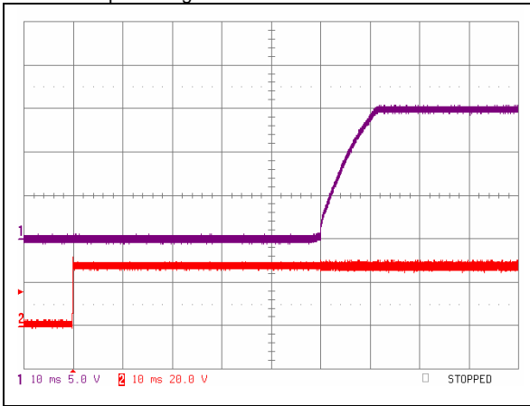
iQE24007A150V-000 Typical startup from input voltage application at full load. Lower trace - input voltage, Upper trace – output voltage. Time scale 10ms/div.
