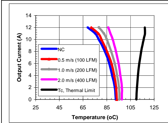
iQE24012A080V-000 maximum output current vs. ambient temperature at nominal input voltage for airflow rates natural convection (60lfm) to 400lfm with airflow from pin 3 to pin 1 (best orientation).
