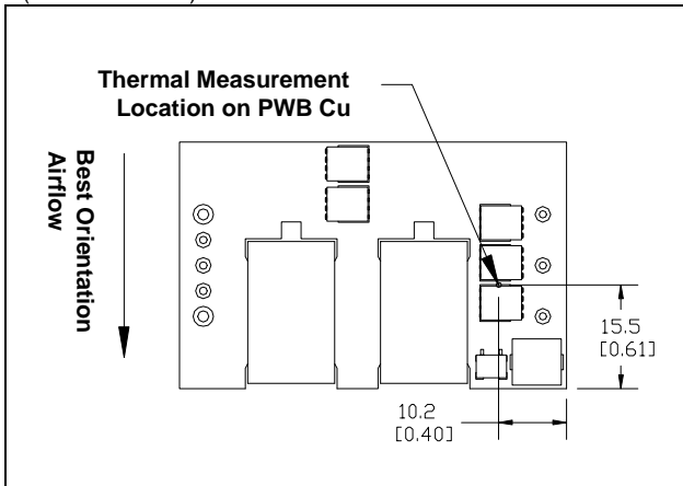
iQE24024A050V-000 thermal measurement location – top view
