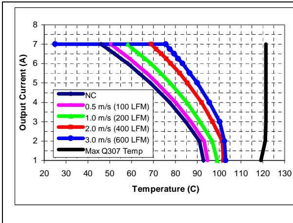
iQE24007A150V-000 maximum output current vs. ambient temperature at nominal input voltage for airflow rates natural convection (60lfm) to 600lfm with airflow from pin 3 to pin 1 (best orientation).
