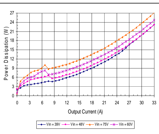
Power Dissipation vs. Vin (test in socket, no base-plate)
