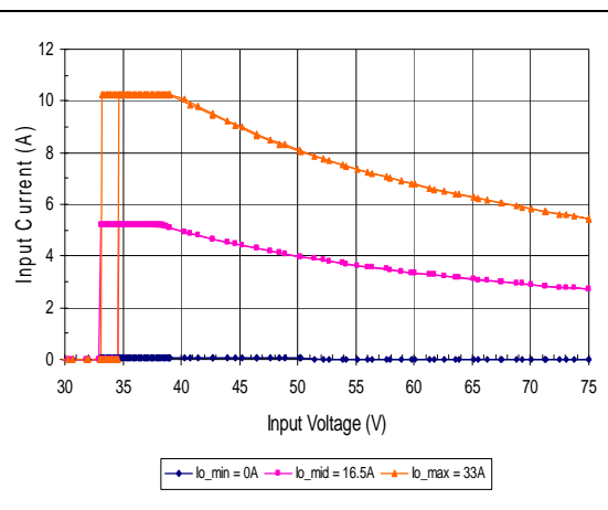
Typical Input Current vs. Input Voltage Characteristics
