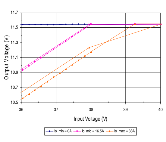
Output Voltage vs. Vin (between 36V and 40V)
