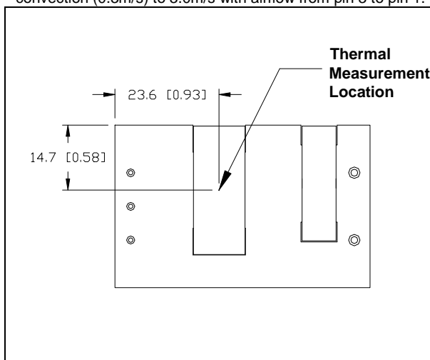
Thermal measurement location – top view
