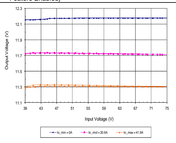
Output Voltage vs. Input Voltage (Droop Feature Enabled)
