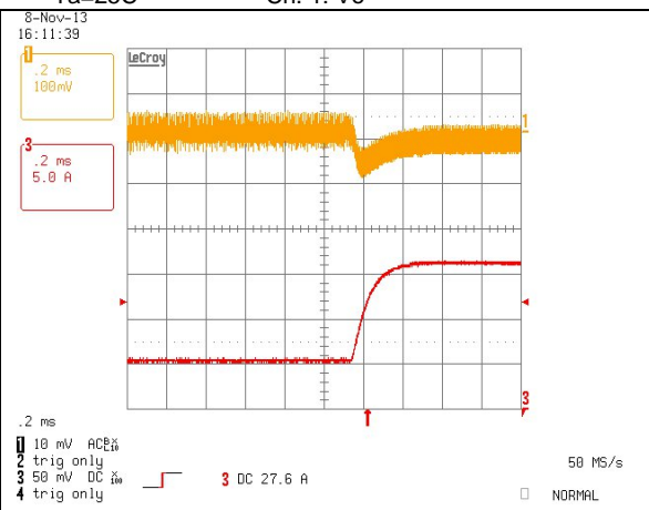
Load Transient Response (Droop disabled) 50% to 75% of Load with di/dt= 0.1A/uS. Ch. 1: Vo Ch. 3: Io
