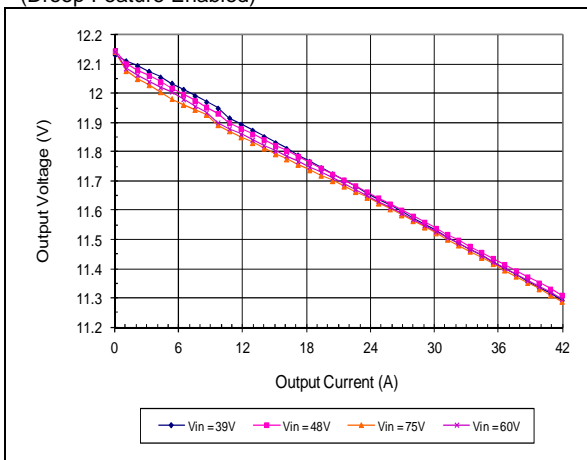
Output Voltage vs. Load Current (Droop Feature Enabled)
