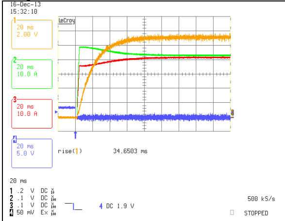
Start-up from on/off switch: 54Vin, Io=84A (200% Load) Ch. 1: Vo Ch. 2: Io1 Ch. 3: Io2 Ch. 4: ON/OFF
