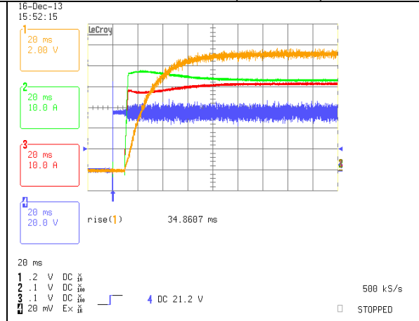
Start-up from Vin: 54Vin, Io=84A (200% Load) Ch. 1: Vo Ch. 2: Io1 Ch. 3: Io2 Ch. 4: Vin
