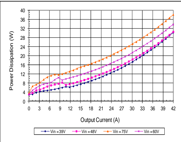
Power Dissipation vs. Load at Various Vin (tested in socket, voltage droop feature disabled)
