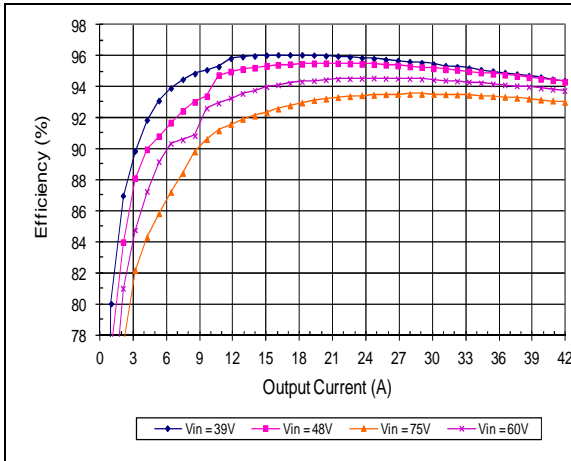
Efficiency vs. Load at Various Vin (tested in socket, voltage droop feature disabled)
