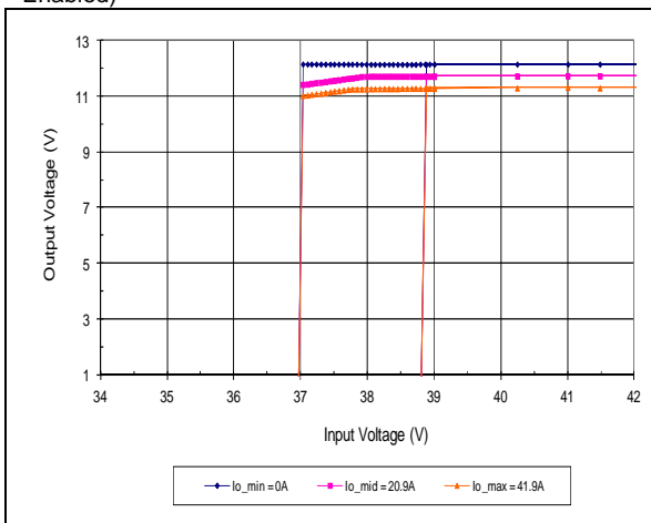
Output Voltage vs. Vin Turn-on and Turn-off at Ta=25C
