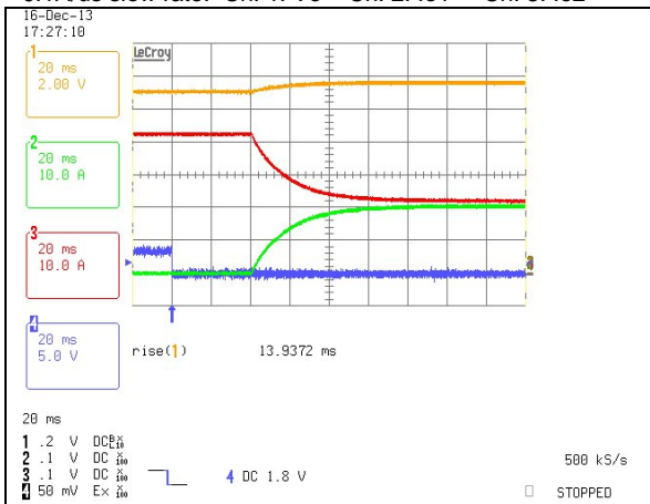
Start-up with back-biasing: Vin=54V, Turn-on 2 nd Unit Ch. 1: Vo Ch. 2: Io1 Ch. 3: Io2 Ch. 4: ON/OFF
