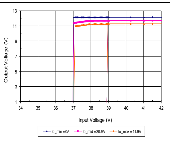
Output Voltage vs. Vin Turn-on and Turn-off at Ta=65C
