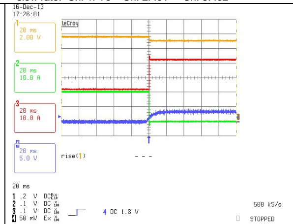
Back-biasing, Vin=54V, Io=42A, Turn-off 2 nd Unit Ch. 1: Vo Ch. 2: Io1 Ch. 3: Io2 Ch. 4: ON/OFF
