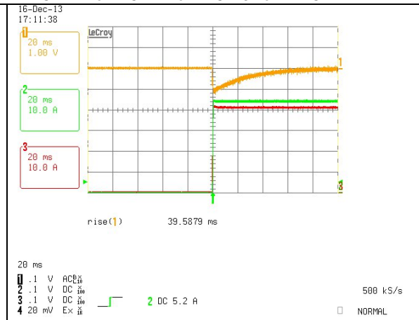
Load Transient Response. Load Step: 0A to 84A, 0.1A/us slew rate. Ch. 1: Vo Ch. 2: Io1 Ch. 3: Io2
