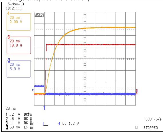
Start-up from on/off Switch at Vin,nom and Full Load. Ch. 1: Vo Ch. 3: Io Ch. 4: ON/OFF
