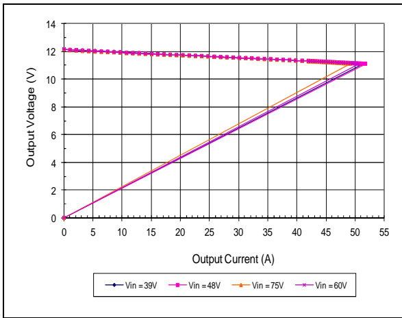
Output Current Limit Characteristics vs. Input Voltage (Droop Feature Enabled)
