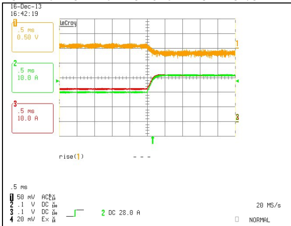
Load Transient Response. Load Step: 42A to 63A, 0.1A/us slew rate. Ch. 1: Vo Ch. 2: Io1 Ch. 3: Io2
