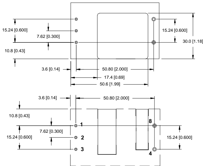
Recommended hole pattern (top view)
