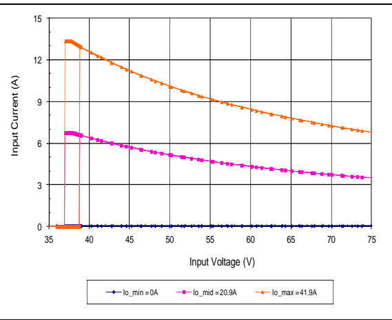
Input Current vs. Input Voltage Characteristics (Droop Feature Enabled)
