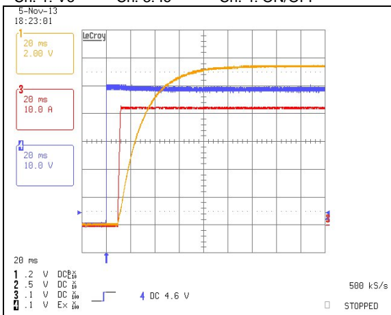
Start-up from Input Voltage Application at Full Load. Ch. 1: Vo Ch. 3: Io Ch. 4: Vin
