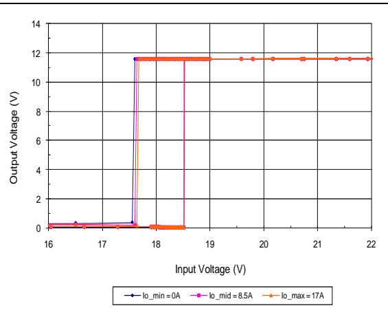
Output Voltage vs. Low Voltage Input Turn-on and off
