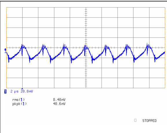
iSA48025A033V-000 Typical Output Ripple at nominal input voltage and full load at Ta=25 degrees; 20mV/div, 2µS/div.
