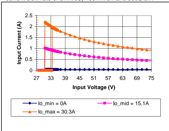
iSA48030A018V-000 Typical Input Current vs. Input Voltage Characteristics
