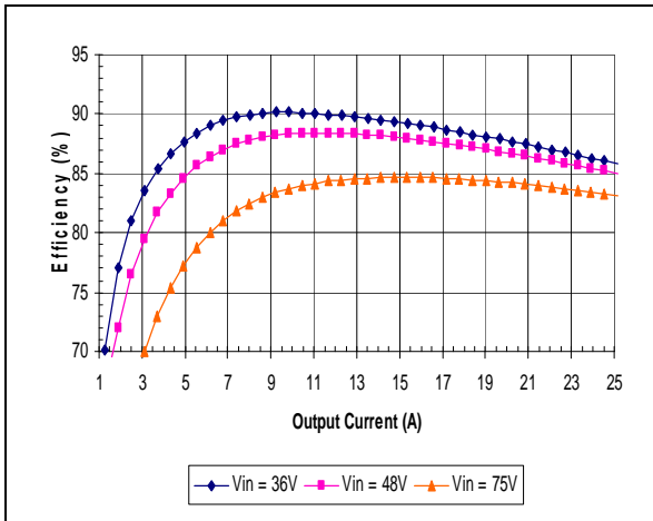
iSA48025A025V-000 Typical Efficiency vs. Input Voltage at Ta=25 degrees.
