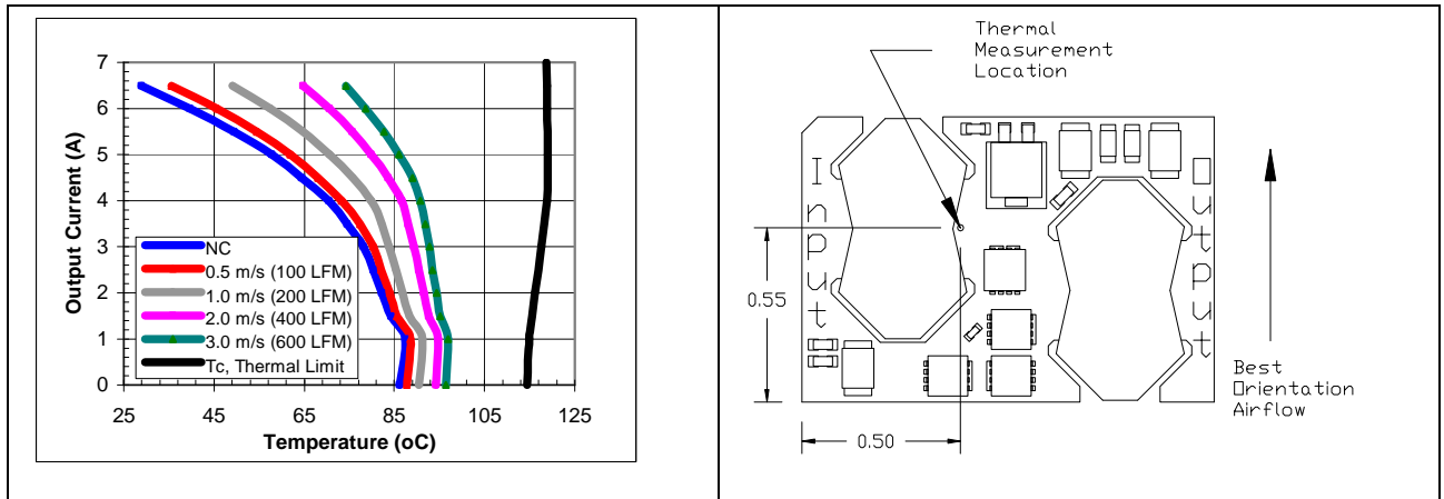
iSA48007A120V-000 maximum output current vs. ambient temperature at nominal input voltage for airflow rates natural convection (60lfm) to 600lfm with airflow from pin 3 to pin 1.
