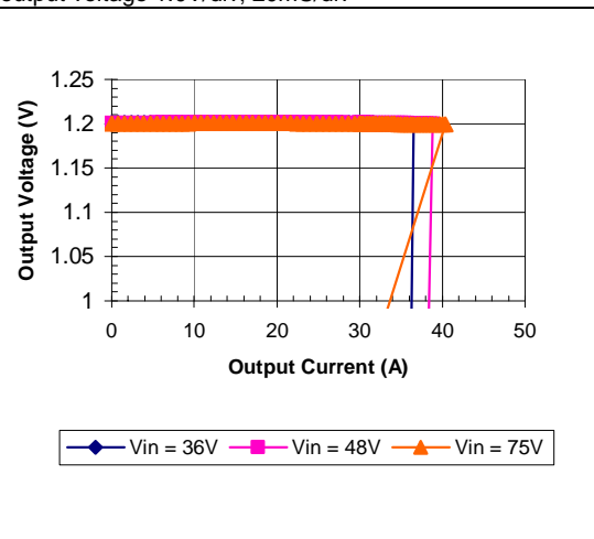
iSA48030A012V-000 Typical Output Current Limit Characteristics vs. Input Voltage at T_a=25 degrees.
