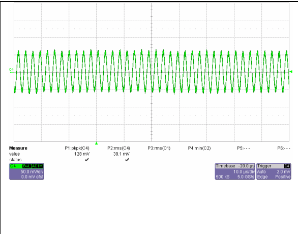
iSA48007A120V-000 Typical Output Ripple at nominal input voltage and full load at Ta=25 degrees; 50mV/div and 10 \mu S/div.
