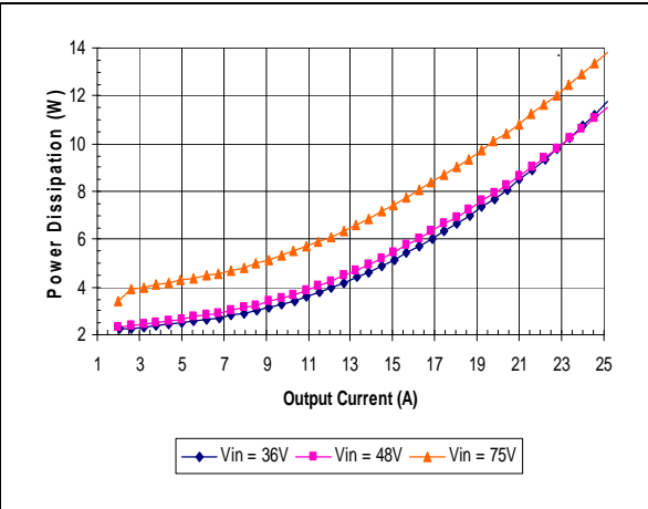
iSA48025A033V-000 Typical Power Dissipation vs. Input Voltage at Ta=25 degrees
