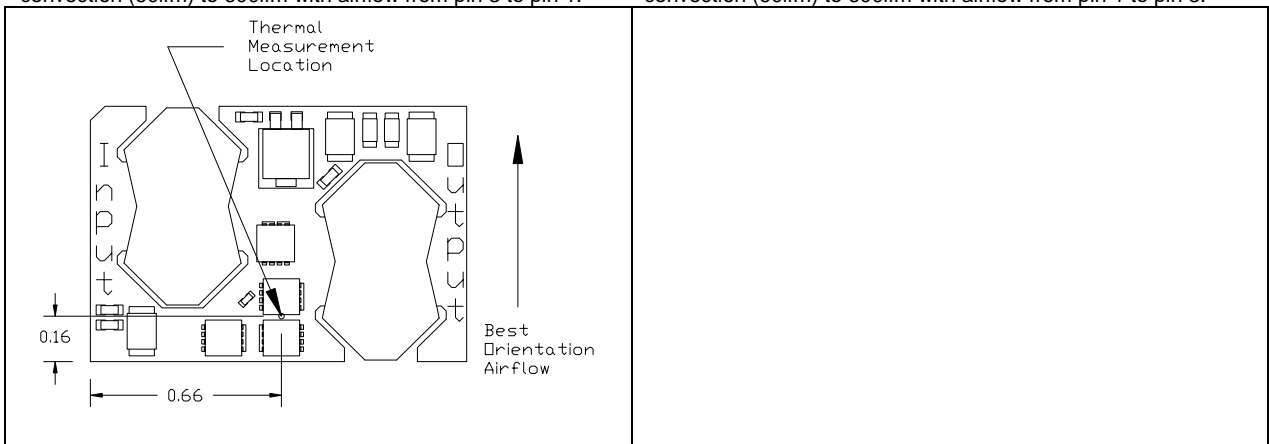
iSA48025A025V-000 thermal measurement location – top view
