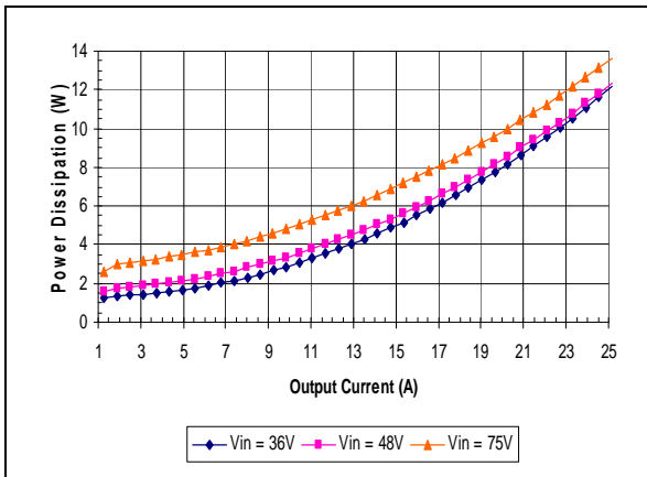
iSA48025A025V-000 Typical Power Dissipation vs. Input Voltage at Ta=85 degrees
