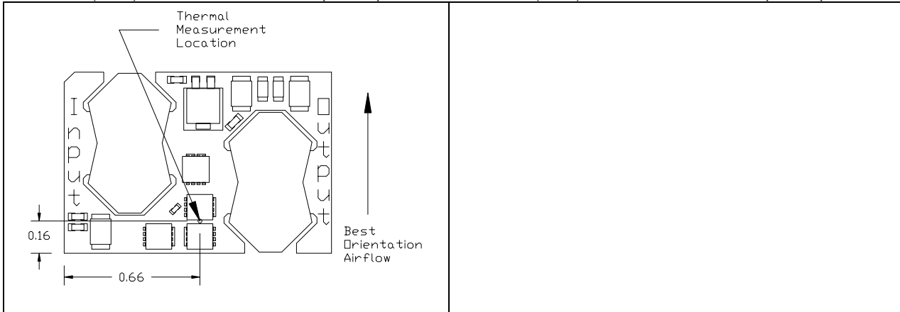
iSA48030A012V-000 thermal measurement location – top view
