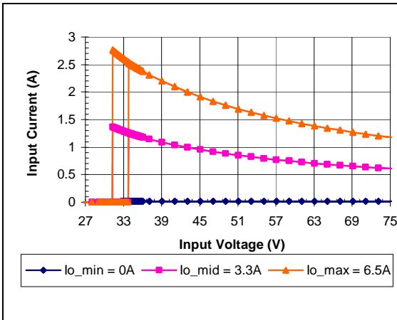
iSA48007A120V-000 Typical Input Current vs. Input Voltage Characteristics
