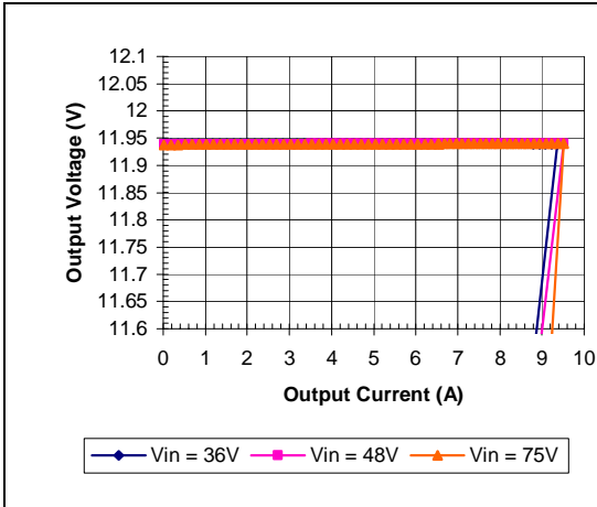
iSA48007A120V-000 Typical Output Current Limit Characteristics vs. Input Voltage at Ta=25 degrees.
