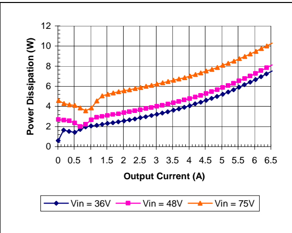
iSA48007A120V-000 Typical Power Dissipation vs. Input Voltage at Ta=25 degrees
