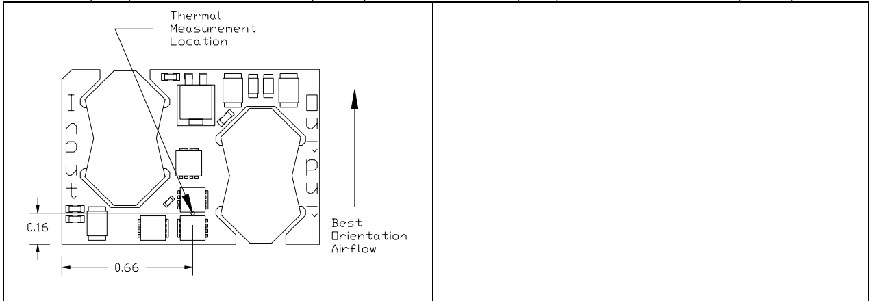
iSA48030A015V-000 thermal measurement location – top view
