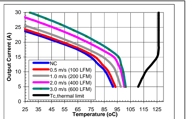
iSA48030A015V-000 maximum output current vs. ambient temperature at nominal input voltage for airflow rates natural convection (60lfm) to 600lfm with airflow from pin 1 to pin 3.
