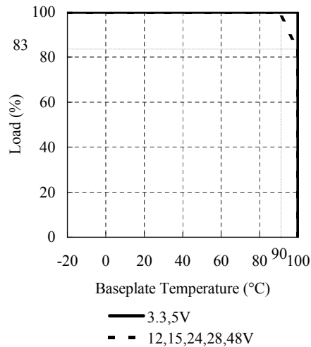
DERATING CURVE
