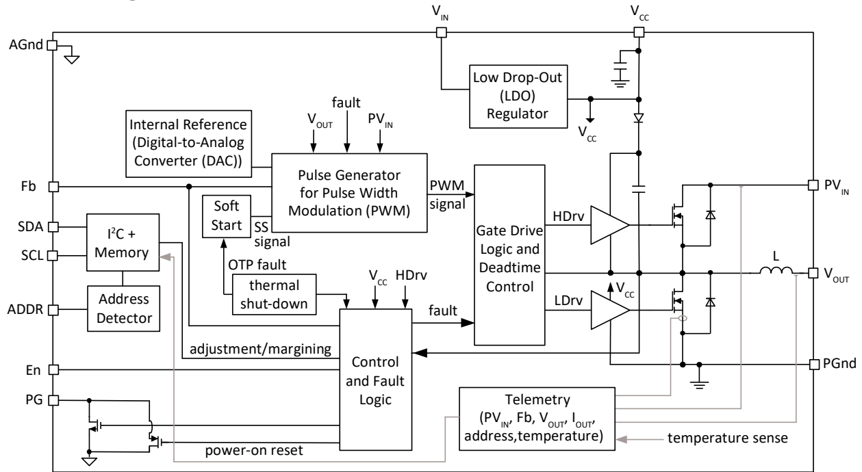
Figure 3 FS1606A \mu POL™
