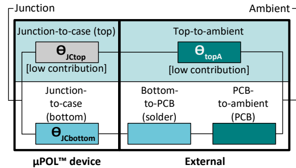
Figure 19 Thermal resistances of the FS1606A
