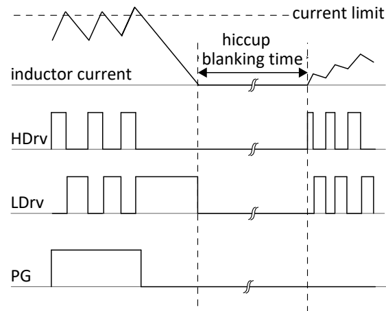
Figure 13 Illustration of OCP in hiccup mode
