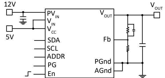
Figure 5 Dual supply applications circuit
