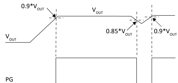
Figure 15 PG signal when PGControl bit=1
