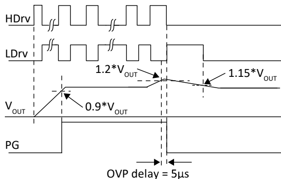
Figure 14 Illustration of latched OVP
