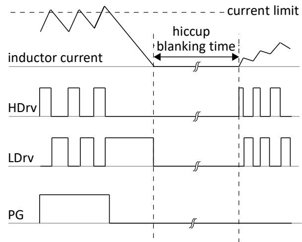
Figure 5 Illustration of OCP in hiccup mode
