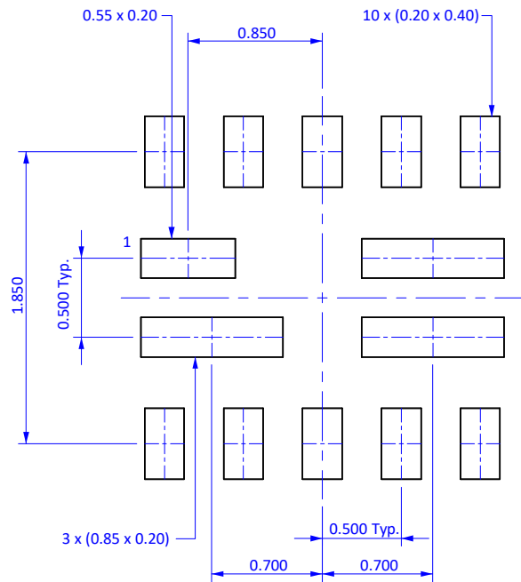
Figure 8 Solder stencil
