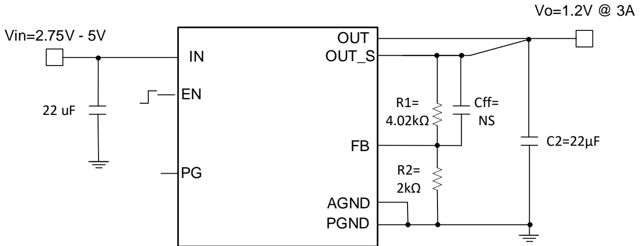
Figure 3 FS3303 application for 1.2V at 3A
