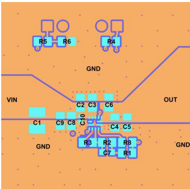
Figure 7 PCB layout
