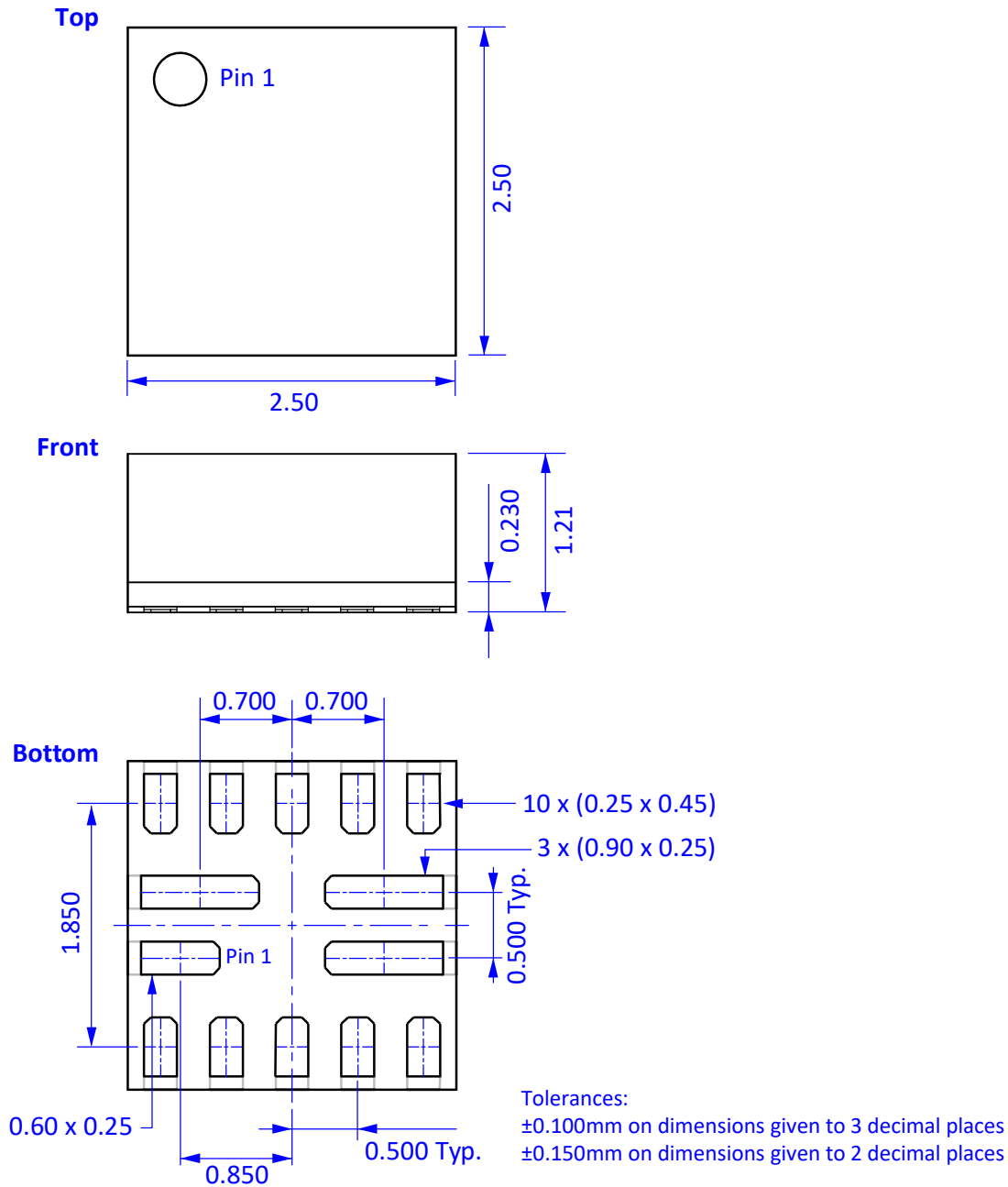
Figure 6 Package outline drawing
