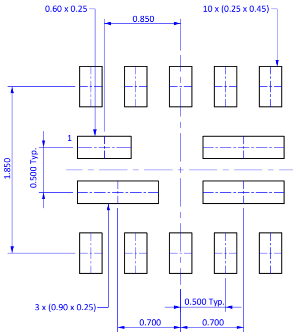
Figure 7 PCB layout
