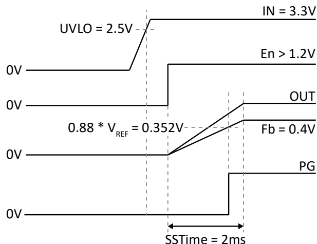
Figure 4 Theoretical operational waveforms during soft-start
