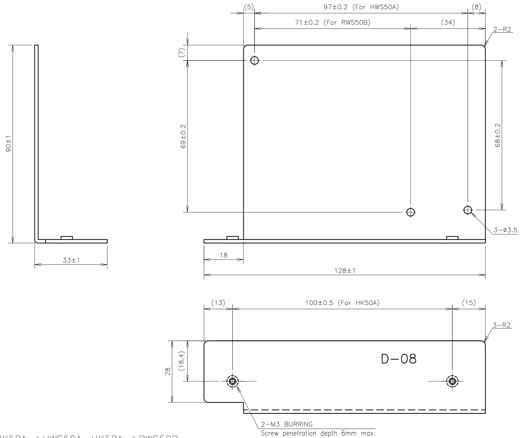
Mounting Plate for HK50A=>HWS50A, HK50A=>RWS50B
