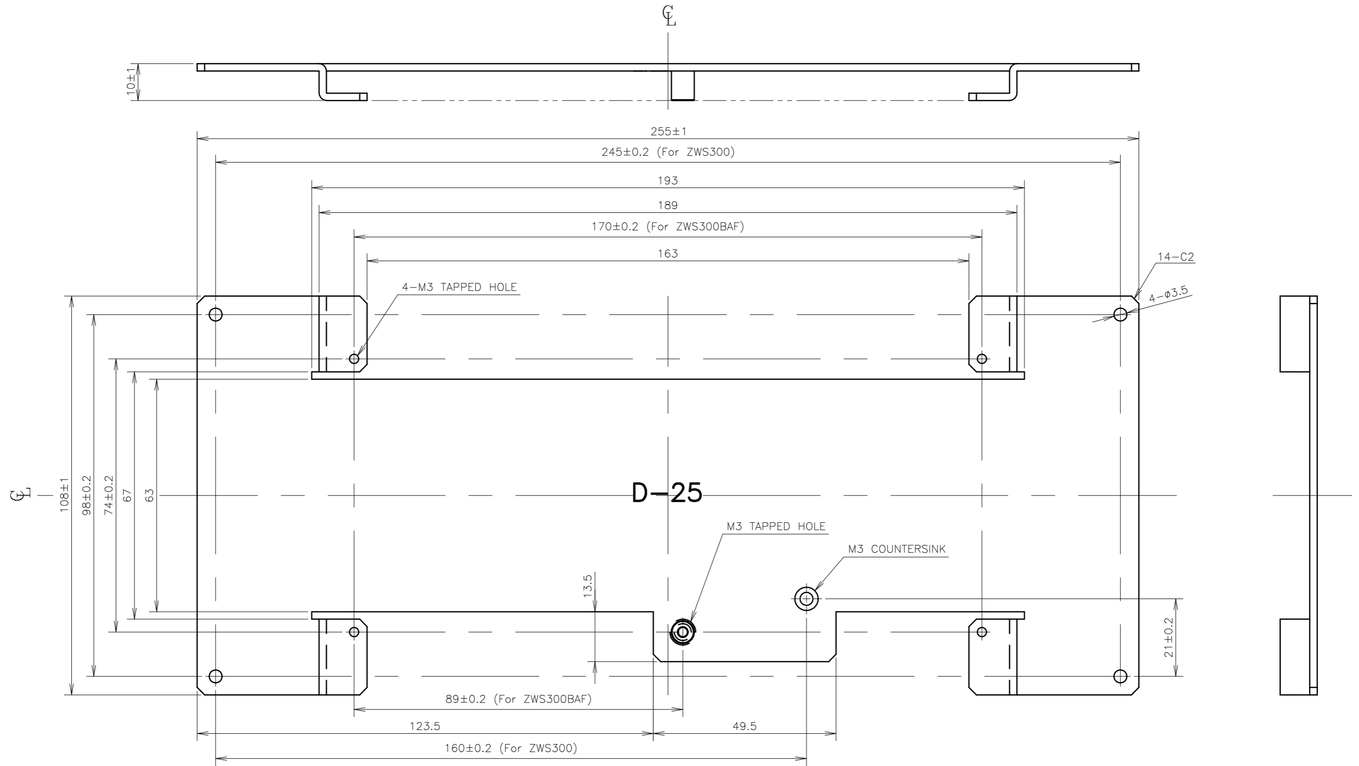
Mounting Plate for ZWS300=>ZWS300BAF
