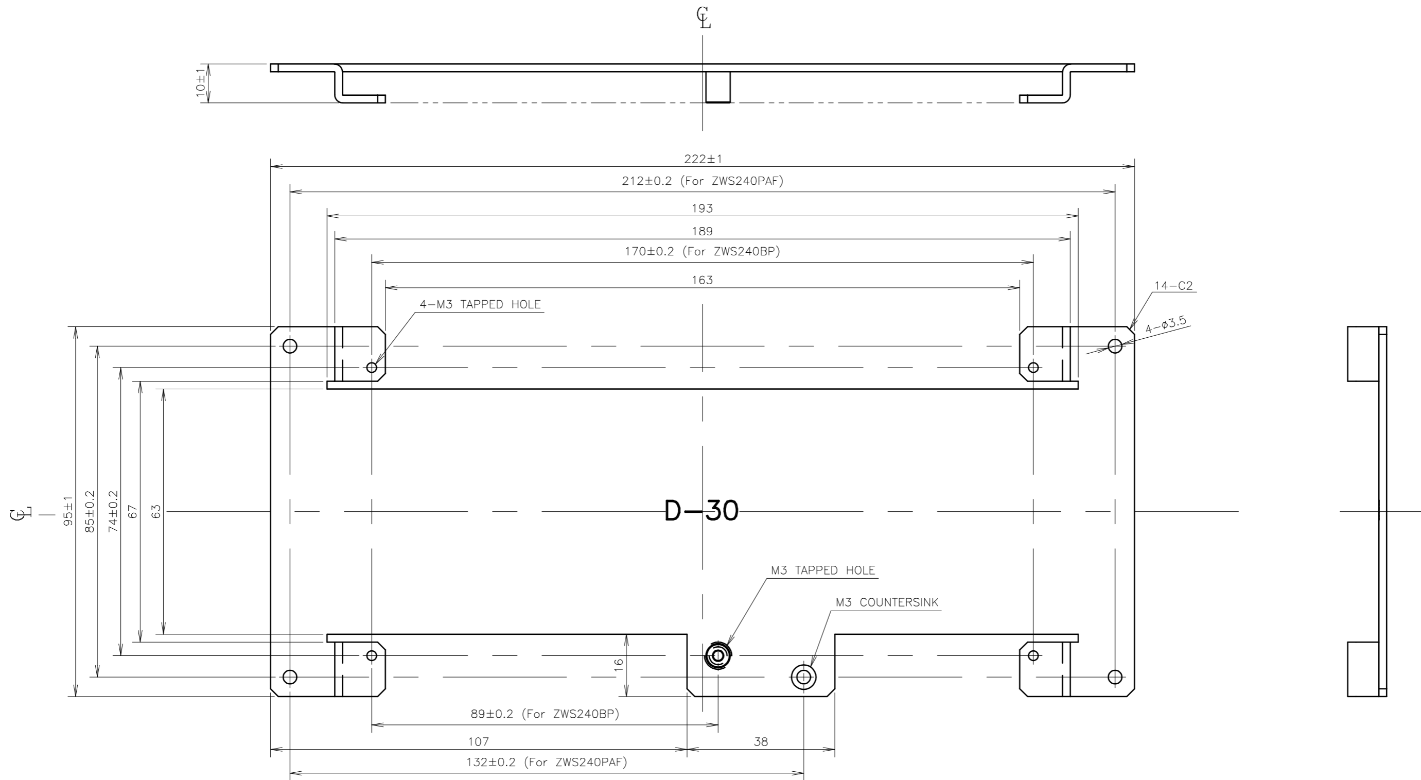
Mounting Plate for ZWS240PAF=>ZWS240BP
