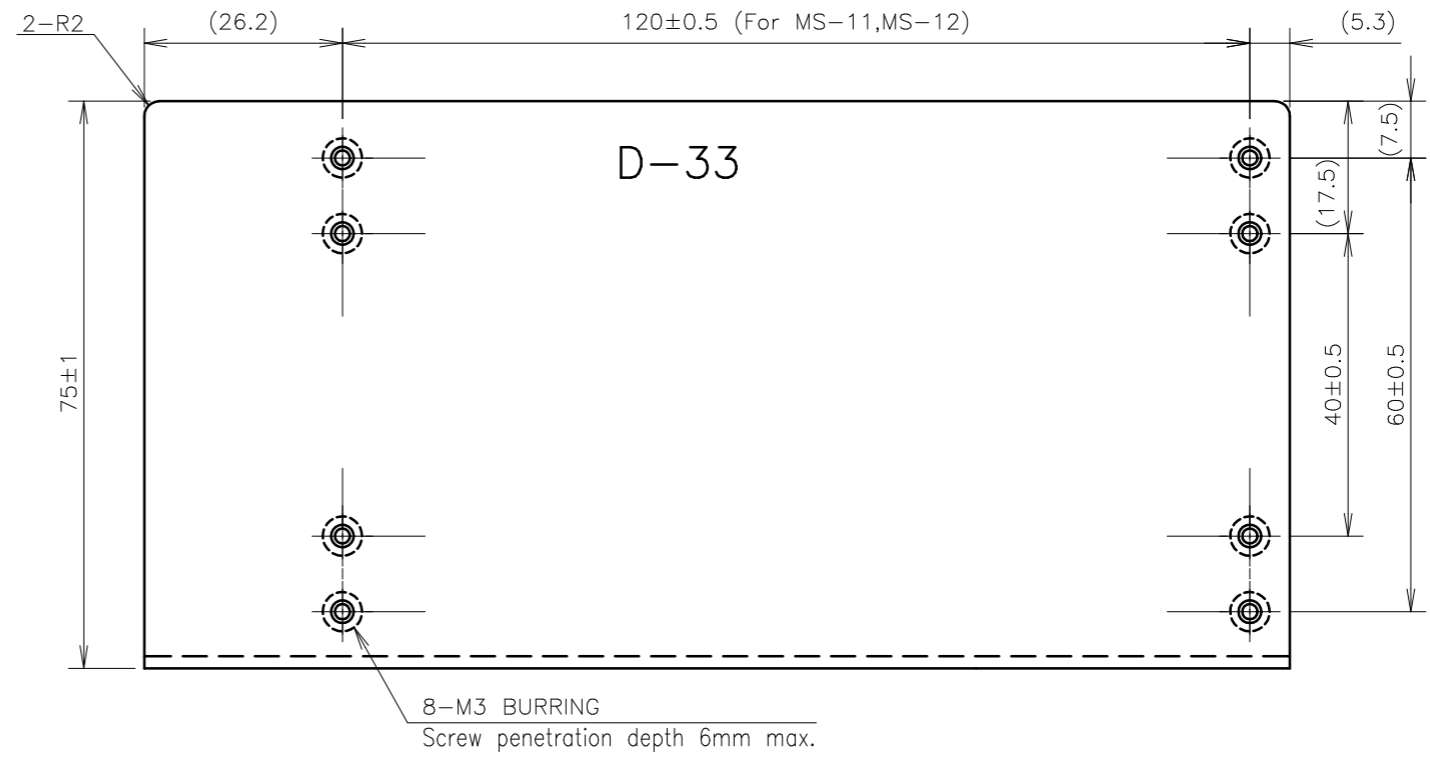
Mounting Plate for MS-11,MS-12=>HMS80,HMS100,HMS150
