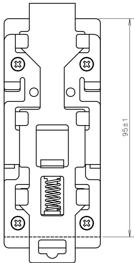
Mounting Plate for HMS50,HWS50A,RWS100B,RWS150B
