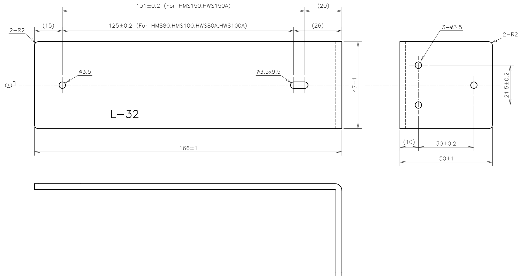
Mounting Plate for HMS80,HMS100,HMS150,HWS80A,HWS100A,HWS150A
