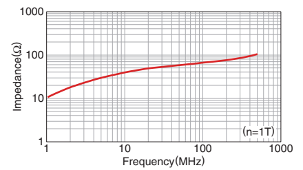
HF70BB9X10X4.5
