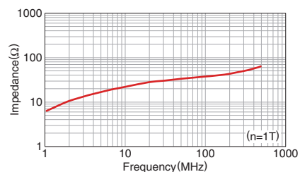
HF70BB5.5X5X2.5
