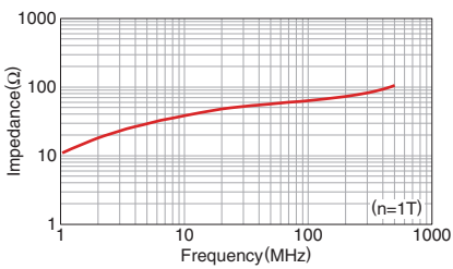
HF70BB6.4X10X3.2
