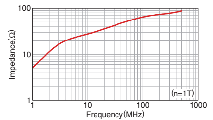
HF57BB3.5X5X1.3
