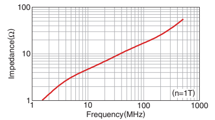
HF57BB3.5X1X1.6
