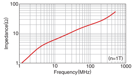
HF57BB3.35X2X2
