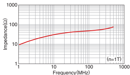
HF70BB1.8X5X0.7
