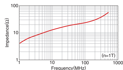
HF70BB3.5X2X1.3
