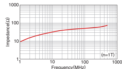
HF70BB4.5X5X1.6
