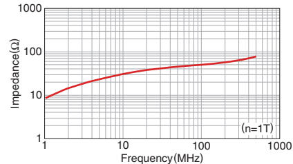
HF70BB2.5X5X0.8
