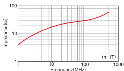
HF70BB4.5X4X2.5
