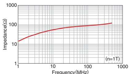
HF70BB3.5X10X1.3
