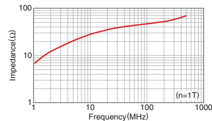
HF70BB3.5X5X1.3
