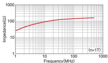
HF70BB4X15X1.35
