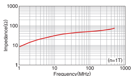
HF70BB3X5X1
